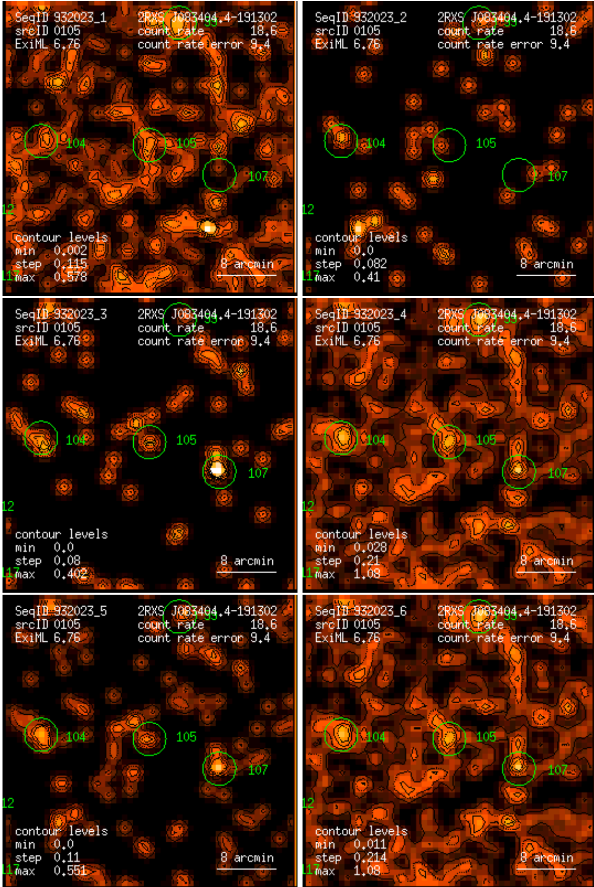
Figure 105: RASS 932023: detection 0105: band rate images, Gaussian filter: (1) PSPC channels 11 – 41, (2) 52 – 90, (3) 91 – 201, (4) 11 – 235, (5) 52 – 201, (6) 11 – 201. Broad band rates in counts/ks. Band rate contour levels in counts/ks/arcmin 2 .
