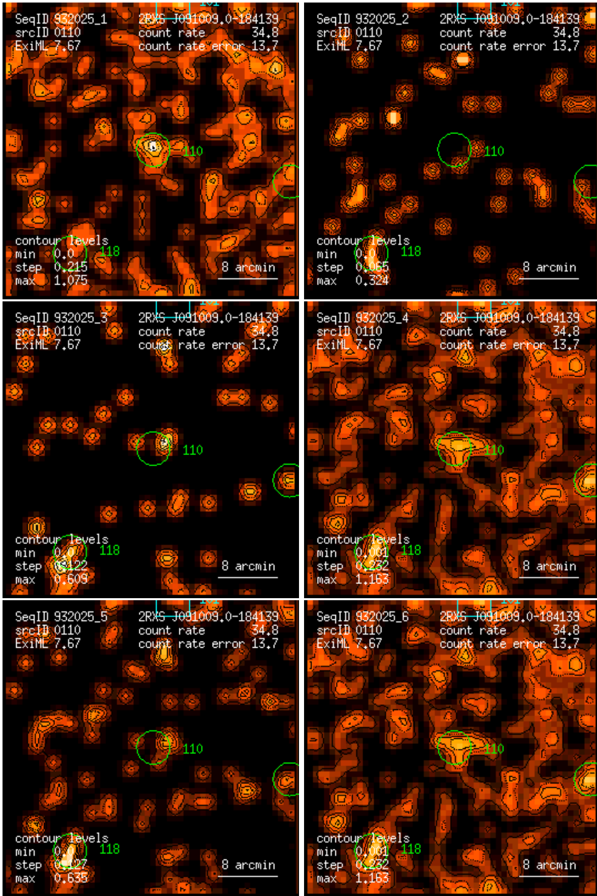
Figure 110: RASS 932025: detection 0110: band rate images, Gaussian filter: (1) PSPC channels 11 – 41, (2) 52 – 90, (3) 91 – 201, (4) 11 – 235, (5) 52 – 201, (6) 11 – 201. Broad band rates in counts/ks. Band rate contour levels in counts/ks/arcmin 2 .
