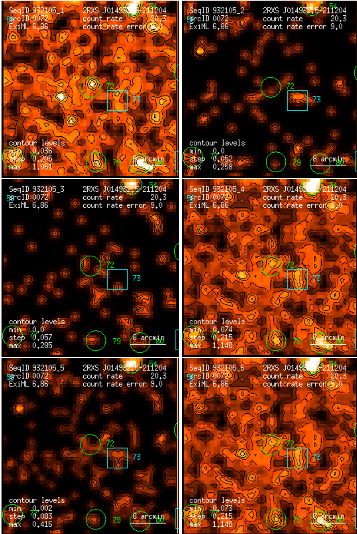
Figure 72: RASS 932105: detection 0072: band rate images, Gaussian filter: (1) PSPC channels 11 – 41, (2) 52 – 90, (3) 91 – 201, (4) 11 – 235, (5) 52 – 201, (6) 11 – 201. Broad band rates in counts/ks. Band rate contour levels in counts/ks/arcmin 2 .
