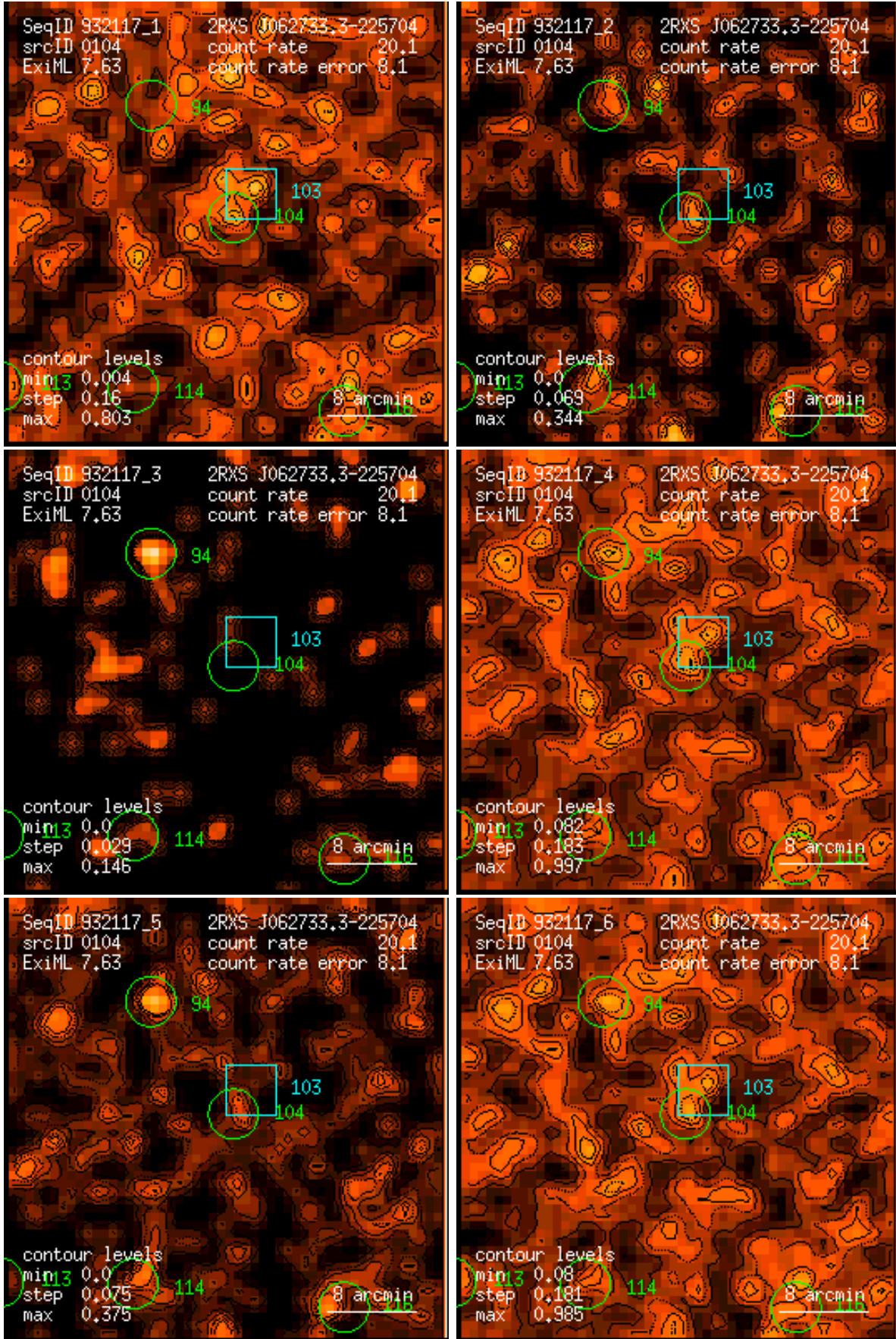
Figure 104: RASS 932117: detection 0104: band rate images, Gaussian filter: (1) PSPC channels 11 – 41, (2) 52 – 90, (3) 91 – 201, (4) 11 – 235, (5) 52 – 201, (6) 11 – 201. Broad band rates in counts/ks. Band rate contour levels in counts/ks/arcmin 2 .
