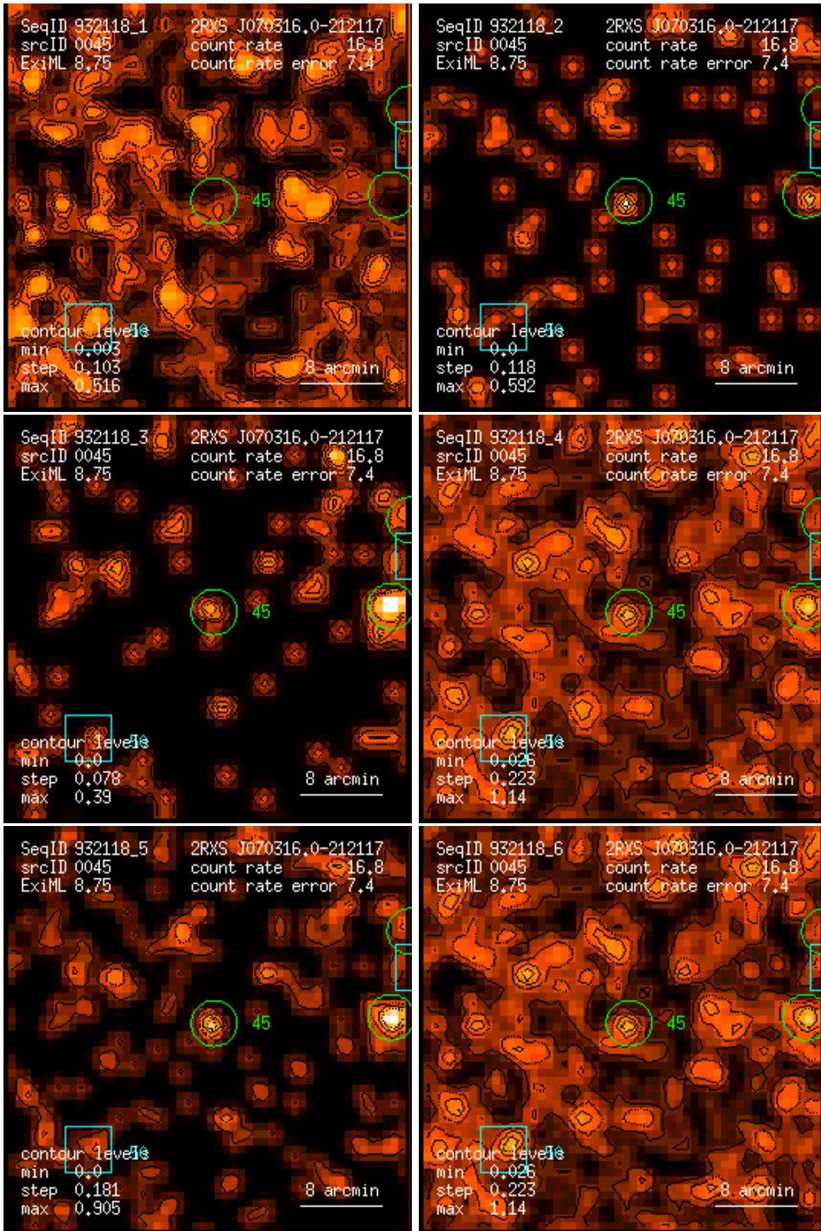
Figure 45: RASS 932118: detection 0045: band rate images, Gaussian filter: (1) PSPC channels 11 – 41, (2) 52 – 90, (3) 91 – 201, (4) 11 – 235, (5) 52 – 201, (6) 11 – 201. Broad band rates in counts/ks. Band rate contour levels in counts/ks/arcmin 2 .
