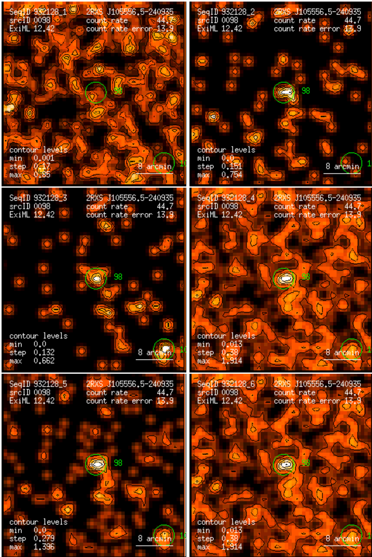
Figure 98: RASS 932128: detection 0098: band rate images, Gaussian filter: (1) PSPC channels 11 – 41, (2) 52 – 90, (3) 91 – 201, (4) 11 – 235, (5) 52 – 201, (6) 11 – 201. Broad band rates in counts/ks. Band rate contour levels in counts/ks/arcmin 2 .
