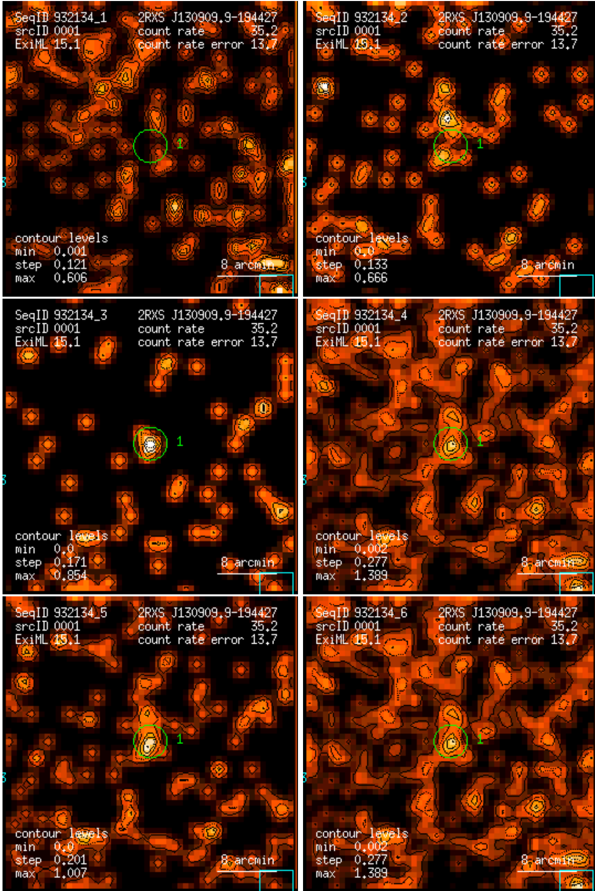
Figure 1: RASS 932134: detection 0001: band rate images, Gaussian filter: (1) PSC channels 11 – 41, (2) 52 – 90, (3) 91 – 201, (4) 11 – 235, (5) 52 – 201, (6) 11 – 201. Broad band rates in counts/ks. Band rate contour levels in counts/ks/arcmin 2 .
