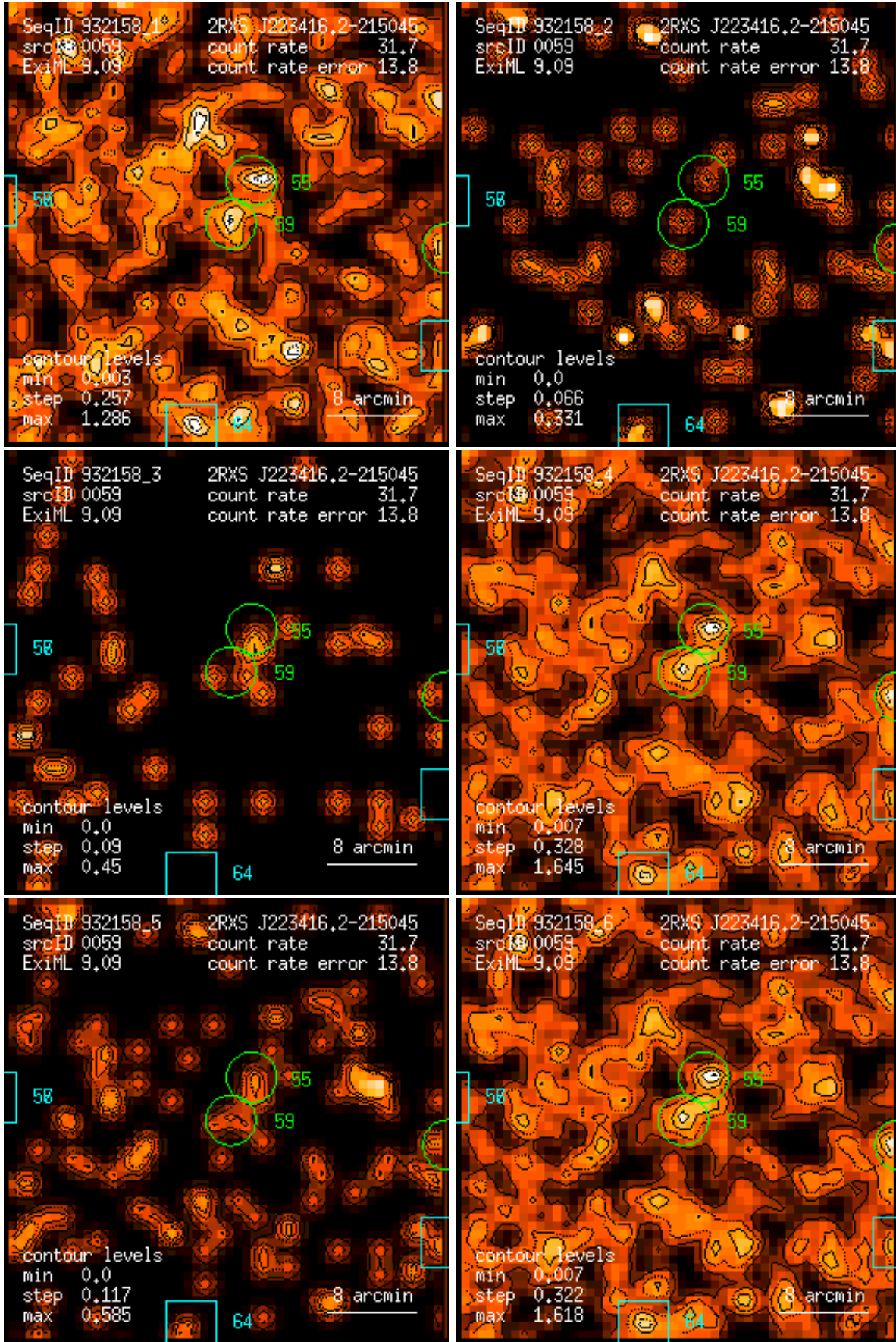
Figure 59: RASS 932158: detection 0059: band rate images, Gaussian filter: (1) PSPC channels 11 – 41, (2) 52 – 90, (3) 91 – 201, (4) 11 – 235, (5) 52 – 201, (6) 11 – 201. Broad band rates in counts/ks. Band rate contour levels in counts/ks/arcmin 2 .
