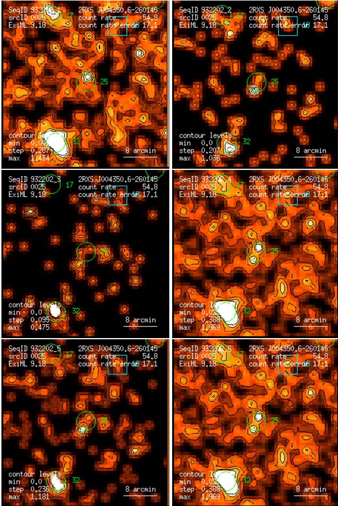
Figure 25: RASS 932202: detection 0025: band rate images, Gaussian filter: (1) PSPC channels 11 – 41, (2) 52 – 90, (3) 91 – 201, (4) 11 – 235, (5) 52 – 201, (6) 11 – 201. Broad band rates in counts/ks. Band rate contour levels in counts/ks/arcmin 2 .
