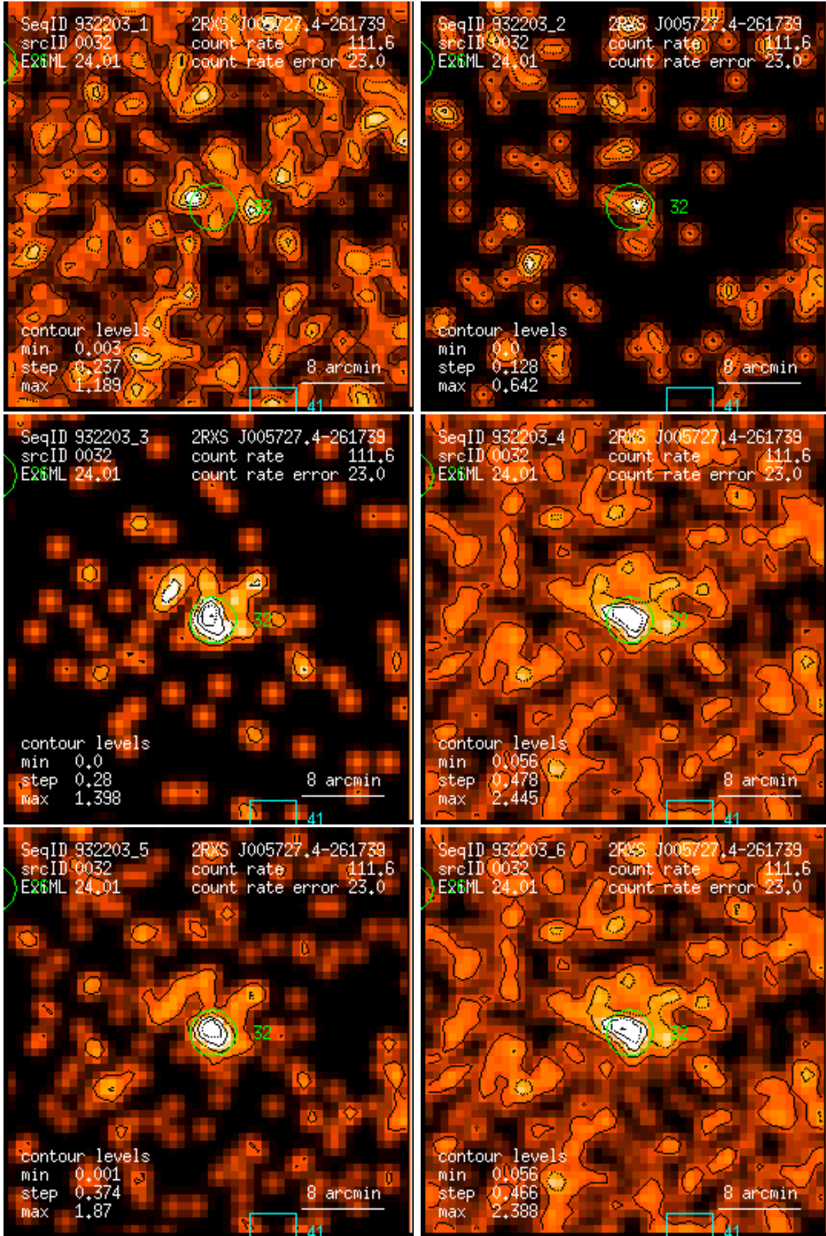
Figure 32: RASS 932203: detection 0032: band rate images, Gaussian filter: (1) PSPC channels 11 – 41, (2) 52 – 90, (3) 91 – 201, (4) 11 – 235, (5) 52 – 201, (6) 11 – 201. Broad band rates in counts/ks. Band rate contour levels in counts/ks/arcmin 2 .
