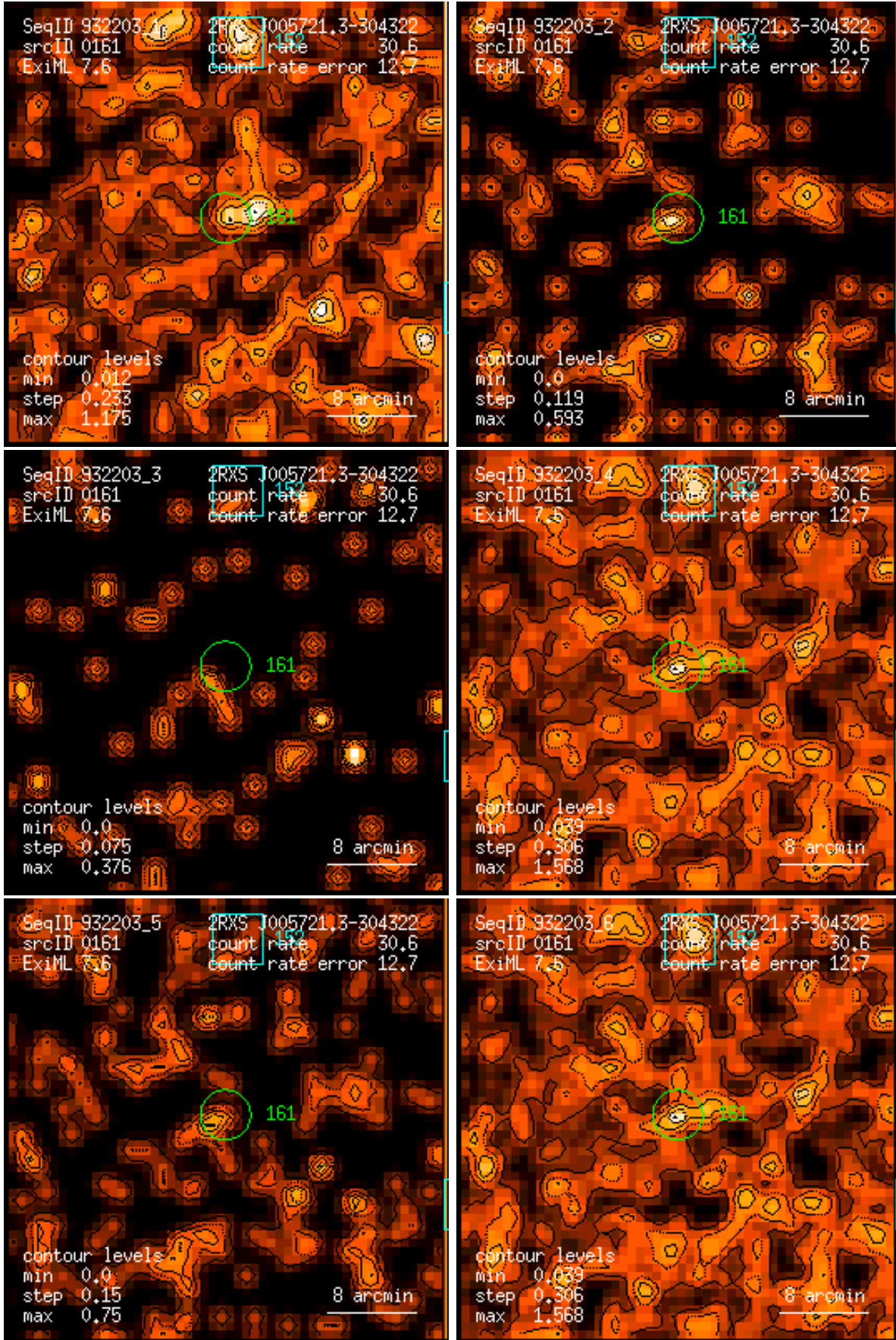
Figure 161: RASS 932203: detection 0161: band rate images, Gaussian filter: (1) PSPC channels 11 – 41, (2) 52 – 90, (3) 91 – 201, (4) 11 – 235, (5) 52 – 201, (6) 11 – 201. Broad band rates in counts/ks. Band rate contour levels in counts/ks/arcmin 2 .
