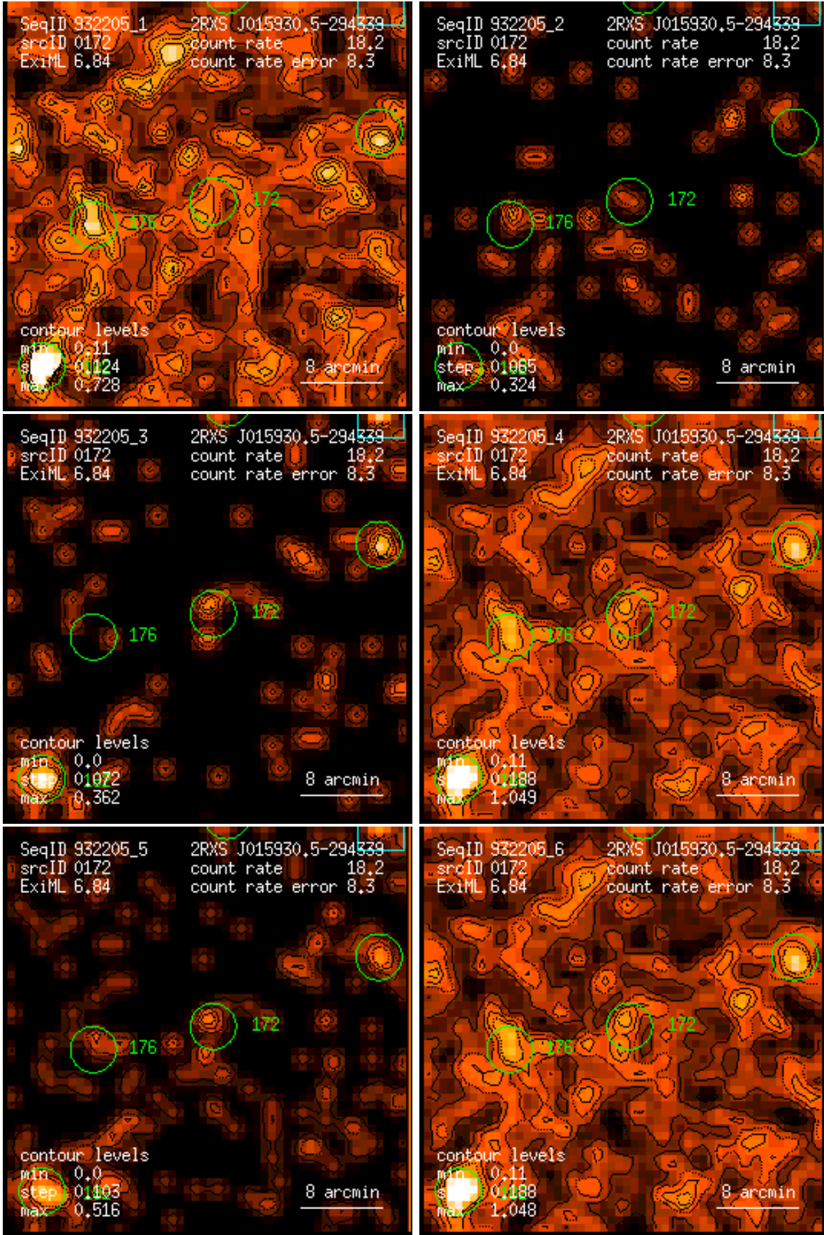
Figure 172: RASS 932205: detection 0172: band rate images, Gaussian filter: (1) PSPC channels 11 – 41, (2) 52 – 90, (3) 91 – 201, (4) 11 – 235, (5) 52 – 201, (6) 11 – 201. Broad band rates in counts/ks. Band rate contour levels in counts/ks/arcmin 2 .
