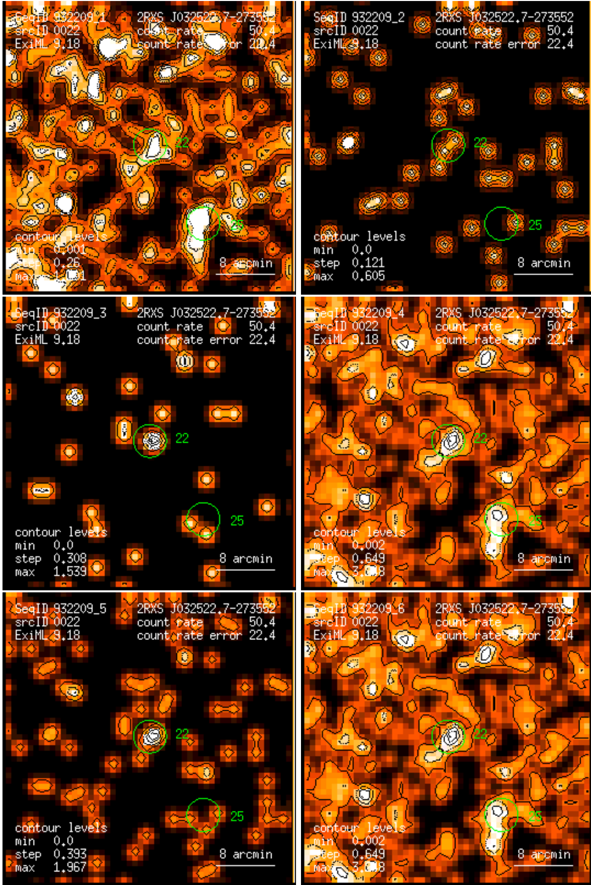
Figure 22: RASS 932209: detection 0022: band rate images, Gaussian filter: (1) PSPC channels 11 – 41, (2) 52 – 90, (3) 91 – 201, (4) 11 – 235, (5) 52 – 201, (6) 11 – 201. Broad band rates in counts/ks. Band rate contour levels in counts/ks/arcmin 2 .
