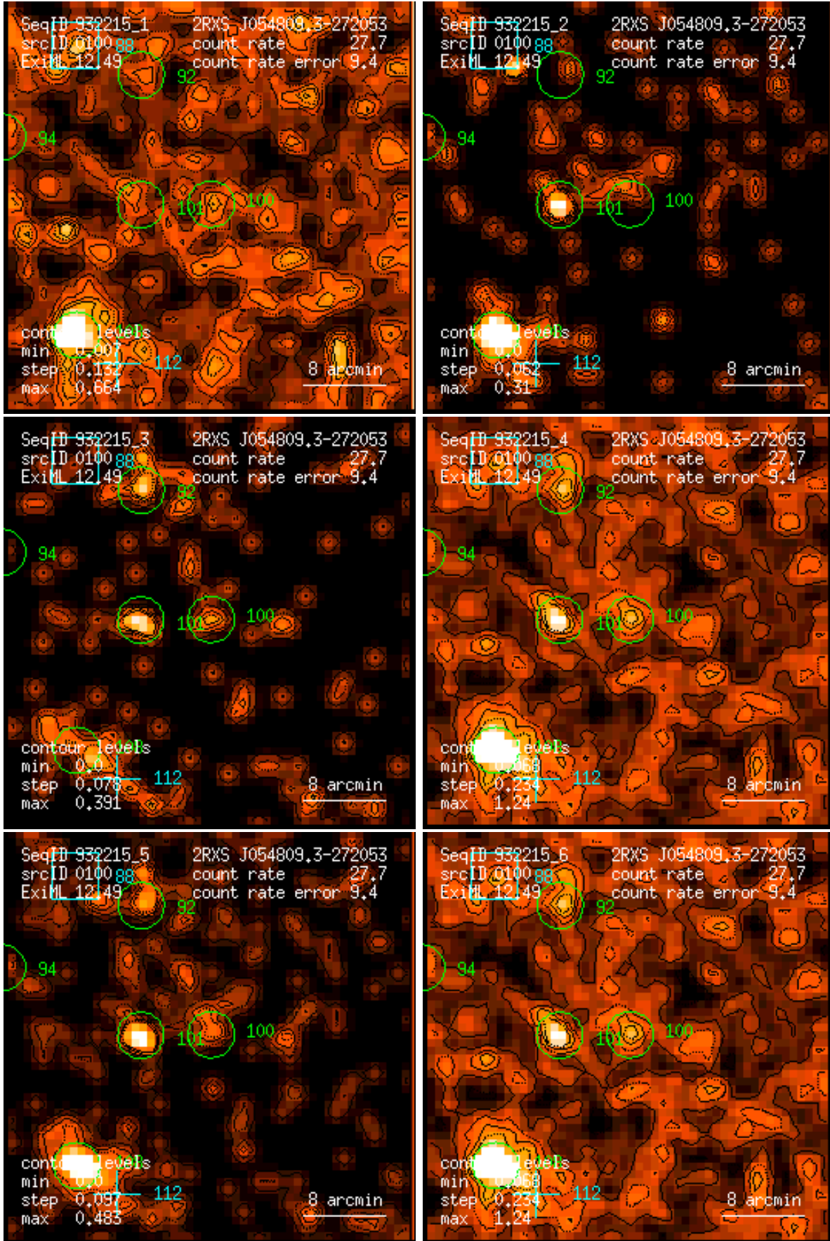
Figure 100: RASS 932215: detection 0100: band rate images, Gaussian filter: (1) PSPC channels 11 – 41, (2) 52 – 90, (3) 91 – 201, (4) 11 – 235, (5) 52 – 201, (6) 11 – 201. Broad band rates in counts/ks. Band rate contour levels in counts/ks/arcmin 2 .
