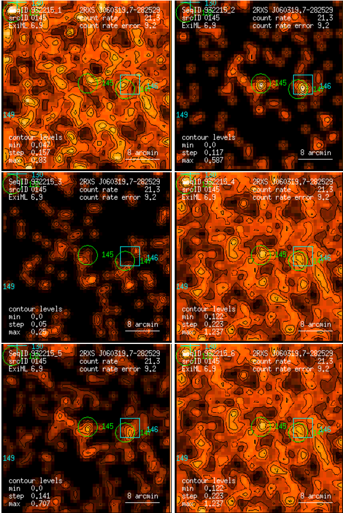
Figure 145: RASS 932215: detection 0145: band rate images, Gaussian filter: (1) PSPC channels 11 – 41, (2) 52 – 90, (3) 91 – 201, (4) 11 – 235, (5) 52 – 201, (6) 11 – 201. Broad band rates in counts/ks. Band rate contour levels in counts/ks/arcmin 2 .
