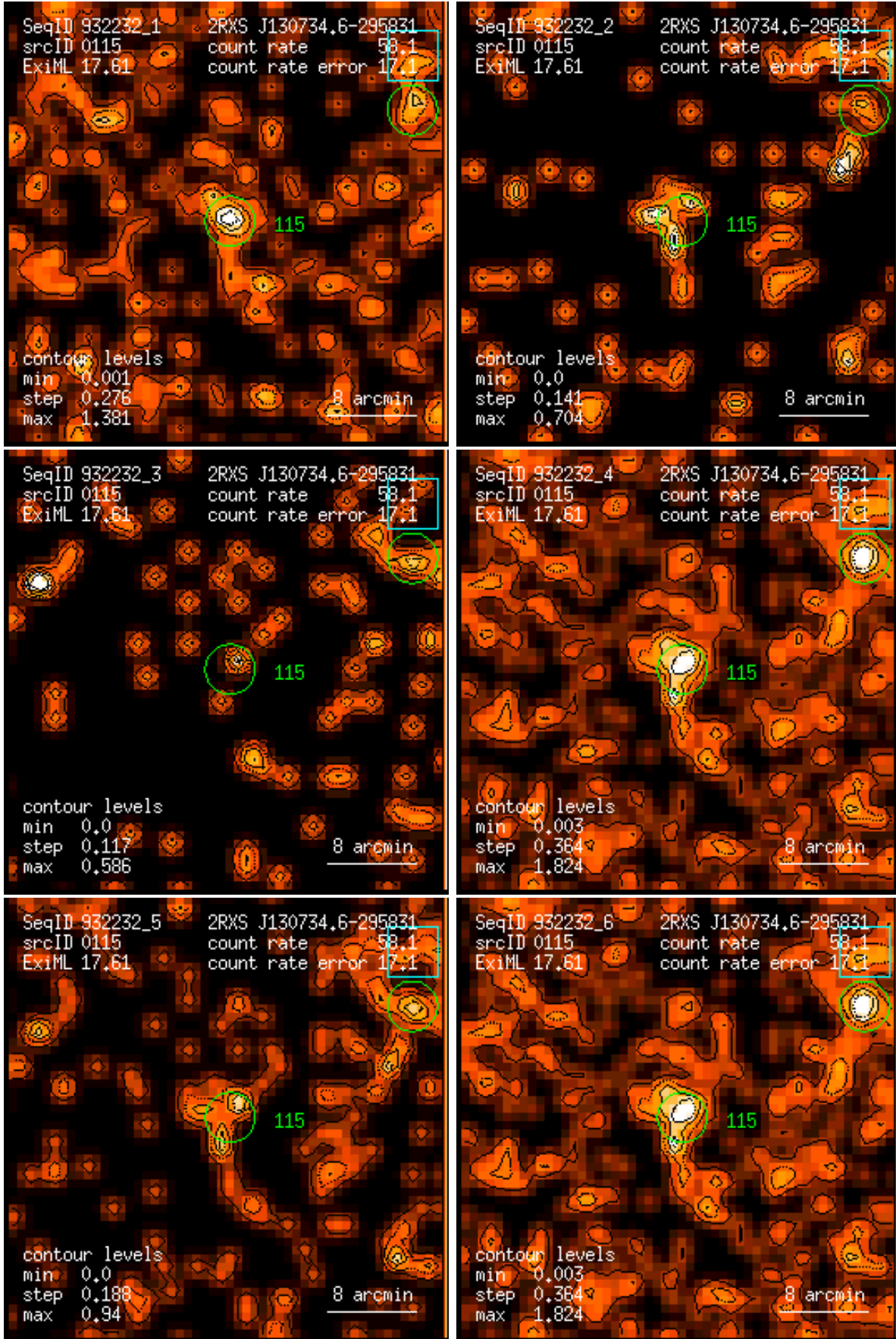
Figure 115: RASS 932232: detection 0115: band rate images, Gaussian filter: (1) PSPC channels 11 – 41, (2) 52 – 90, (3) 91 – 201, (4) 11 – 235, (5) 52 – 201, (6) 11 – 201. Broad band rates in counts/ks. Band rate contour levels in counts/ks/arcmin 2 .
