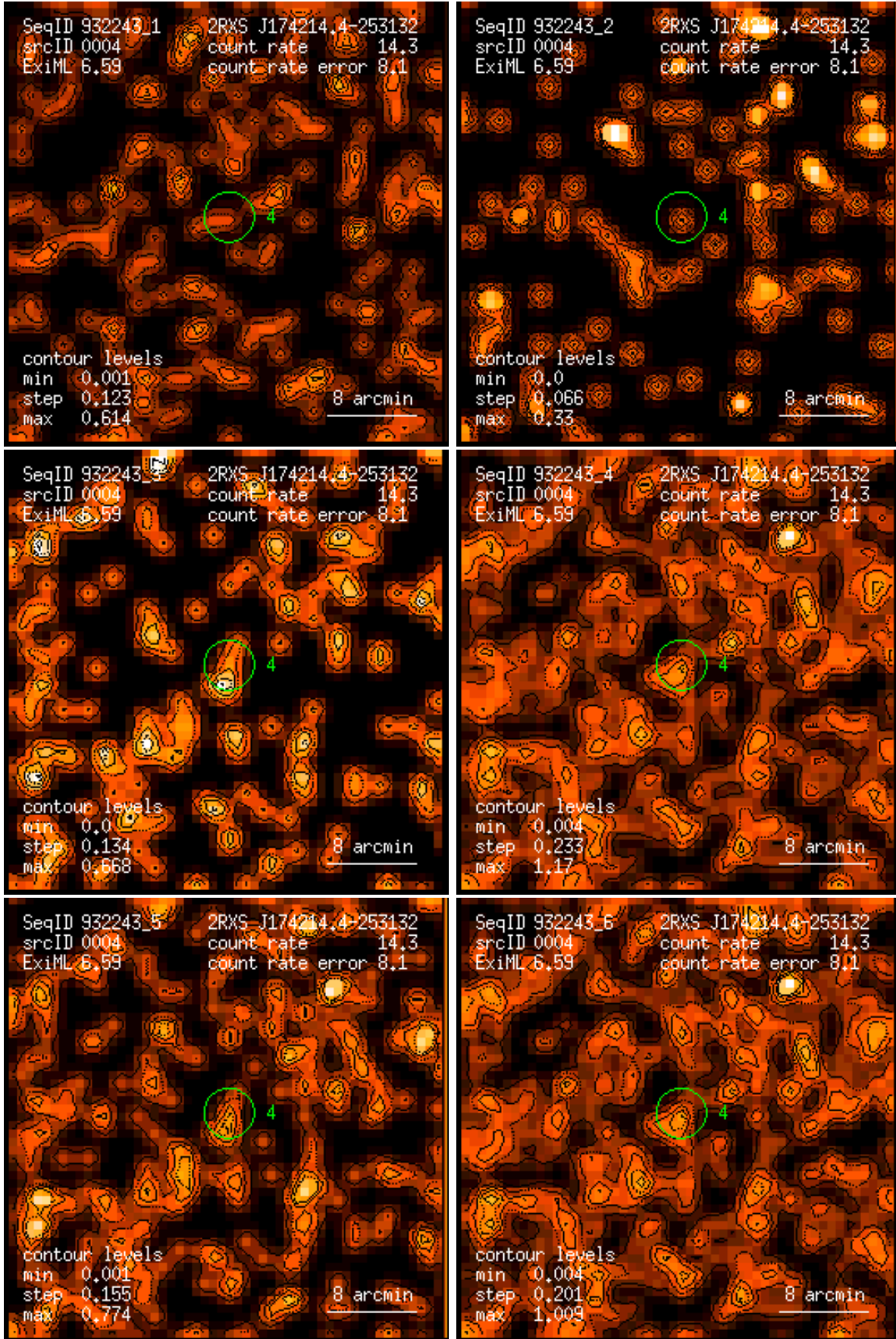
Figure 4: RASS 932243: detection 0004: band rate images, Gaussian filter: (1) PSPC channels 11 – 41, (2) 52 – 90, (3) 91 – 201, (4) 11 – 235, (5) 52 – 201, (6) 11 – 201. Broad band rates in counts/ks. Band rate contour levels in counts/ks/arcmin 2 .
