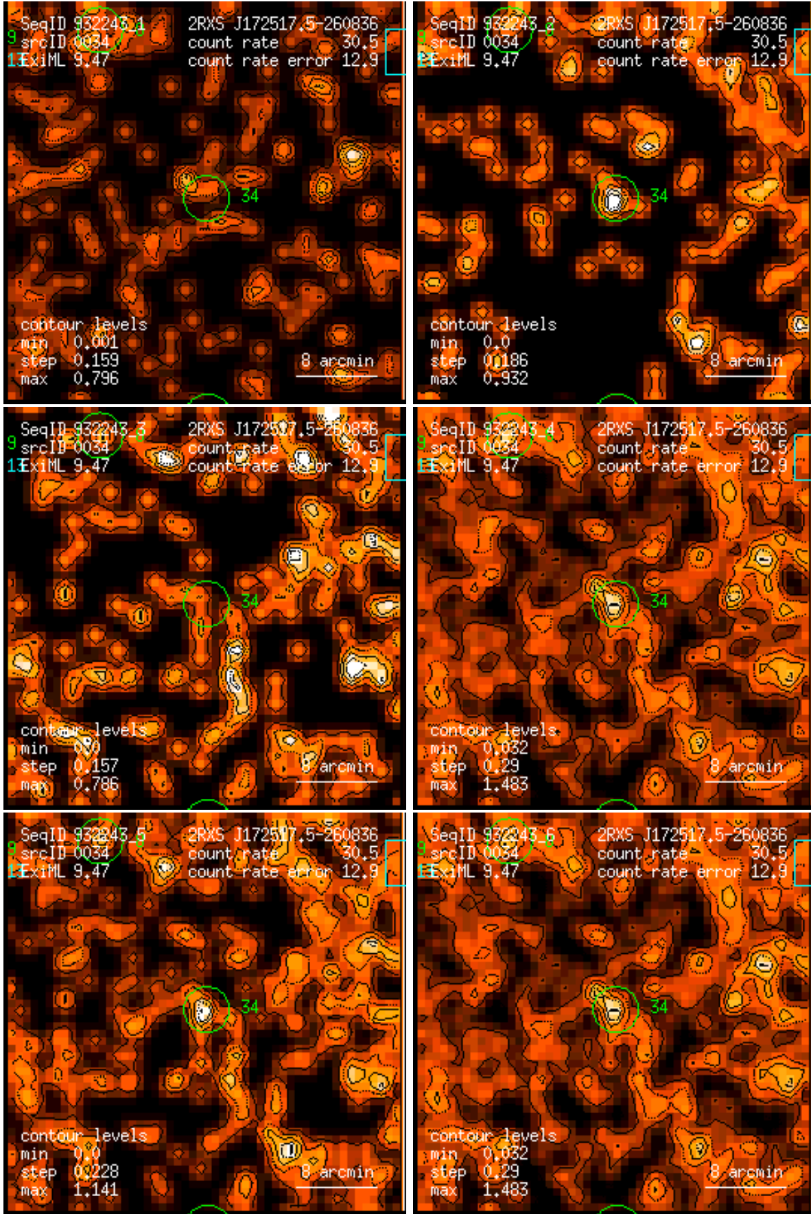
Figure 34: RASS 932243: detection 0034: band rate images, Gaussian filter: (1) PSPC channels 11 – 41, (2) 52 – 90, (3) 91 – 201, (4) 11 – 235, (5) 52 – 201, (6) 11 – 201. Broad band rates in counts/ks. Band rate contour levels in counts/ks/arcmin 2 .
