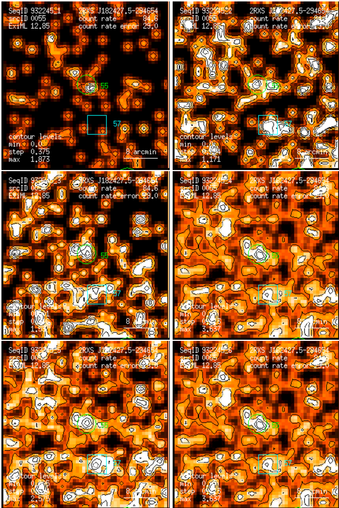
Figure 55: RASS 932245: detection 0055: band rate images, Gaussian filter: (1) PSCC channels 11 – 41, (2) 52 – 90, (3) 91 – 201, (4) 11 – 235, (5) 52 – 201, (6) 11 – 201. Broad band rates in counts/ks. Band rate contour levels in counts/ks/arcmin 2 .
