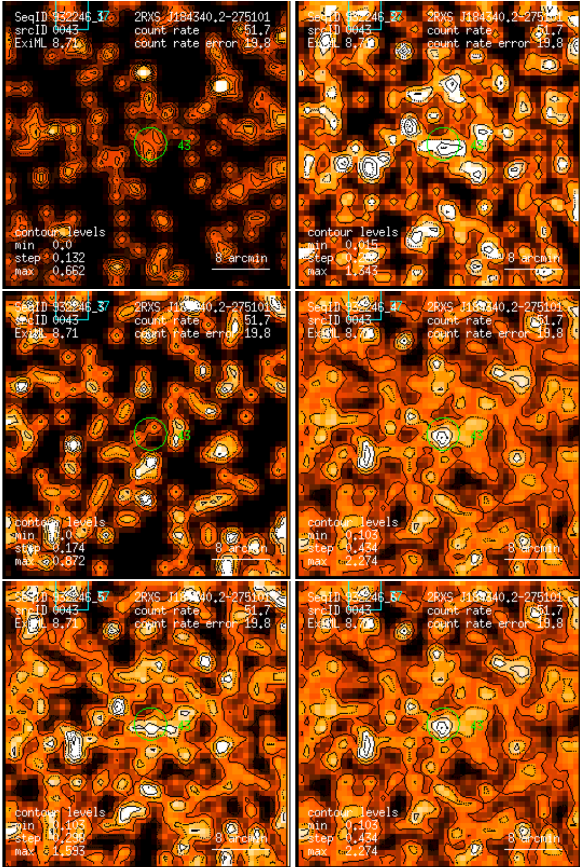
Figure 43: RASS 932246: detection 0043: band rate images, Gaussian filter: (1) PSPC channels 11 – 41, (2) 52 – 90, (3) 91 – 201, (4) 11 – 235, (5) 52 – 201, (6) 11 – 201. Broad band rates in counts/ks. Band rate contour levels in counts/ks/arcmin 2 .
