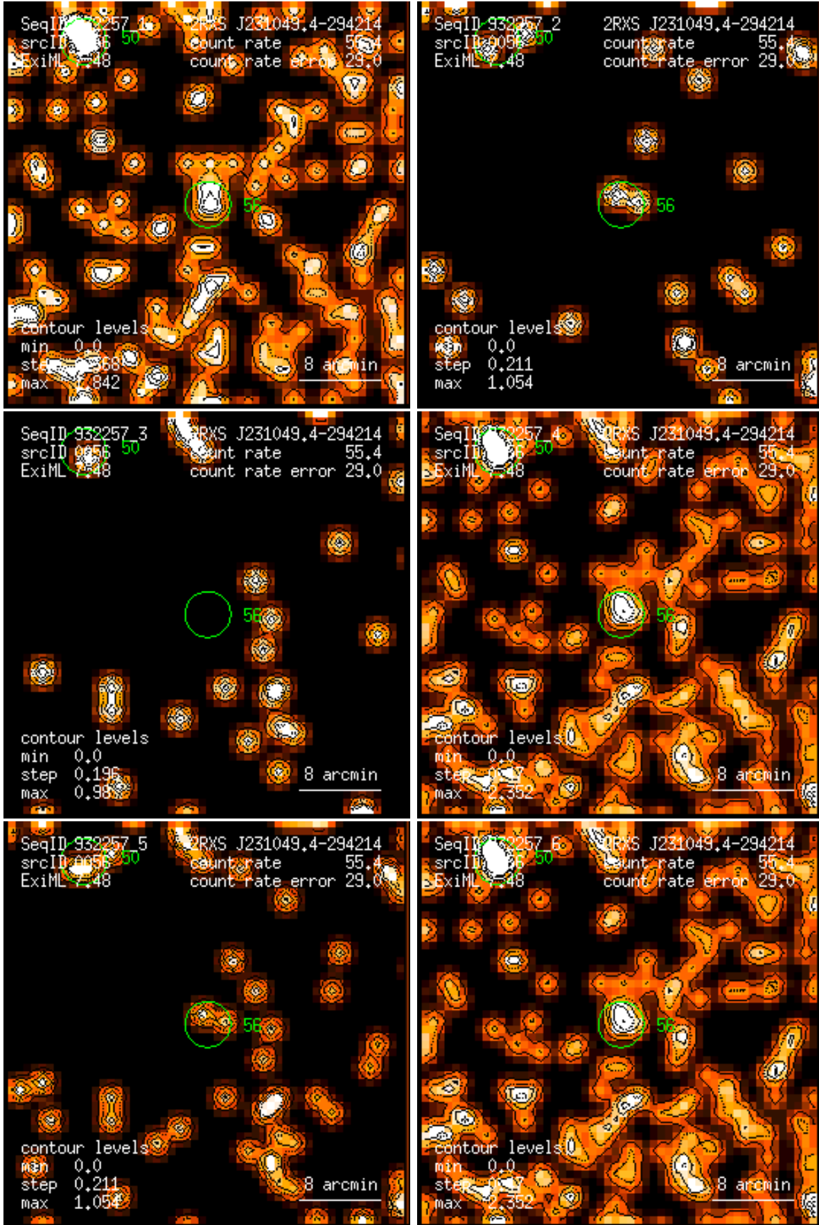
Figure 56: RASS 932257: detection 0056: band rate images, Gaussian filter: (1) PSPC channels 11 – 41, (2) 52 – 90, (3) 91 – 201, (4) 11 – 235, (5) 52 – 201, (6) 11 – 201. Broad band rates in counts/ks. Band rate contour levels in counts/ks/arcmin 2 .
