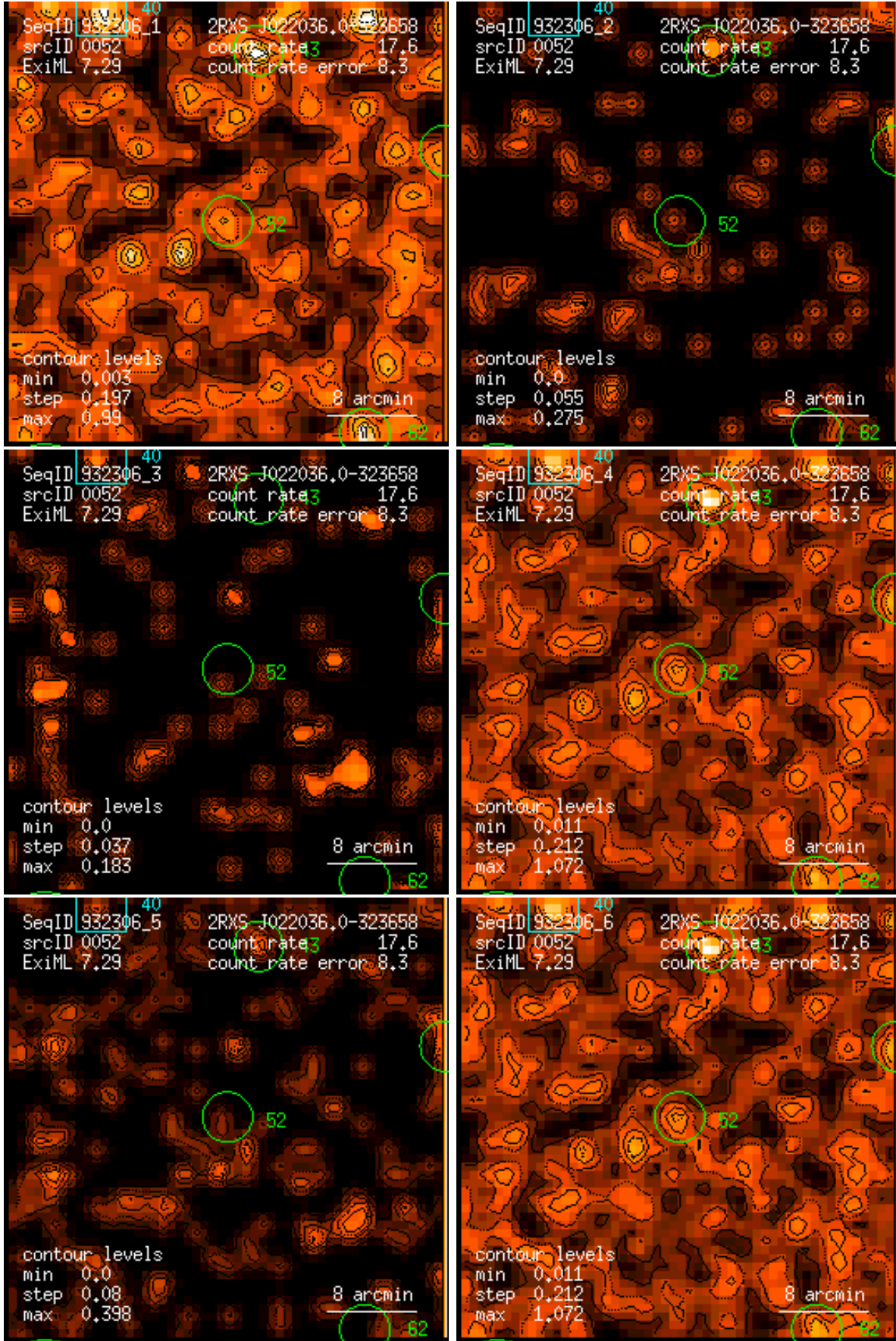
Figure 52: RASS 932306: detection 0052: band rate images, Gaussian filter: (1) PSPC channels 11 – 41, (2) 52 – 90, (3) 91 – 201, (4) 11 – 235, (5) 52 – 201, (6) 11 – 201. Broad band rates in counts/ks. Band rate contour levels in counts/ks/arcmin 2 .
