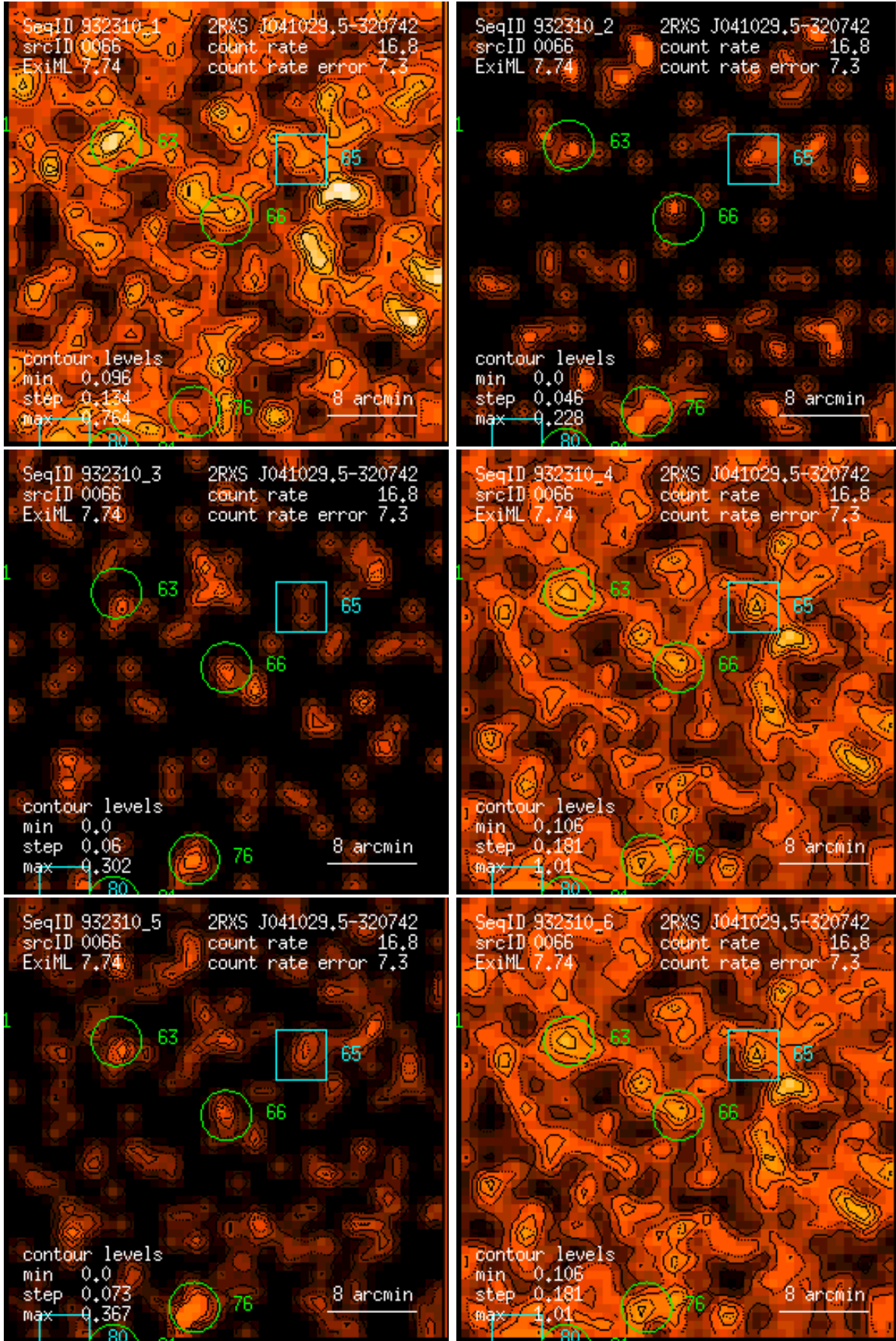
Figure 66: RASS 932310: detection 0066: band rate images, Gaussian filter: (1) PSPC channels 11 – 41, (2) 52 – 90, (3) 91 – 201, (4) 11 – 235, (5) 52 – 201, (6) 11 – 201. Broad band rates in counts/ks. Band rate contour levels in counts/ks/arcmin 2 .
