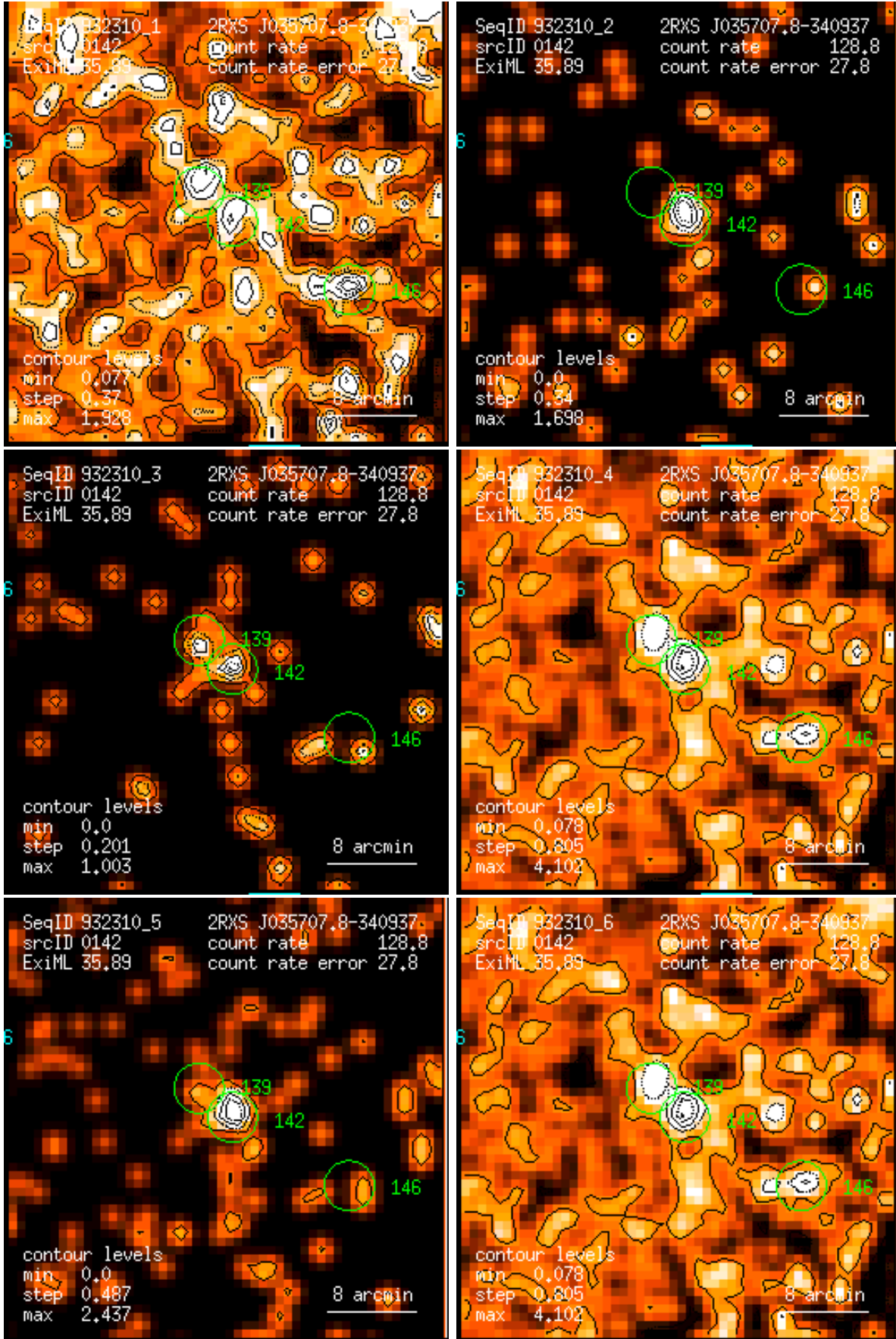
Figure 142: RASS 932310: detection 0142: band rate images, Gaussian filter: (1) PSPC channels 11 – 41, (2) 52 – 90, (3) 91 – 201, (4) 11 – 235, (5) 52 – 201, (6) 11 – 201. Broad band rates in counts/ks. Band rate contour levels in counts/ks/arcmin 2 .
