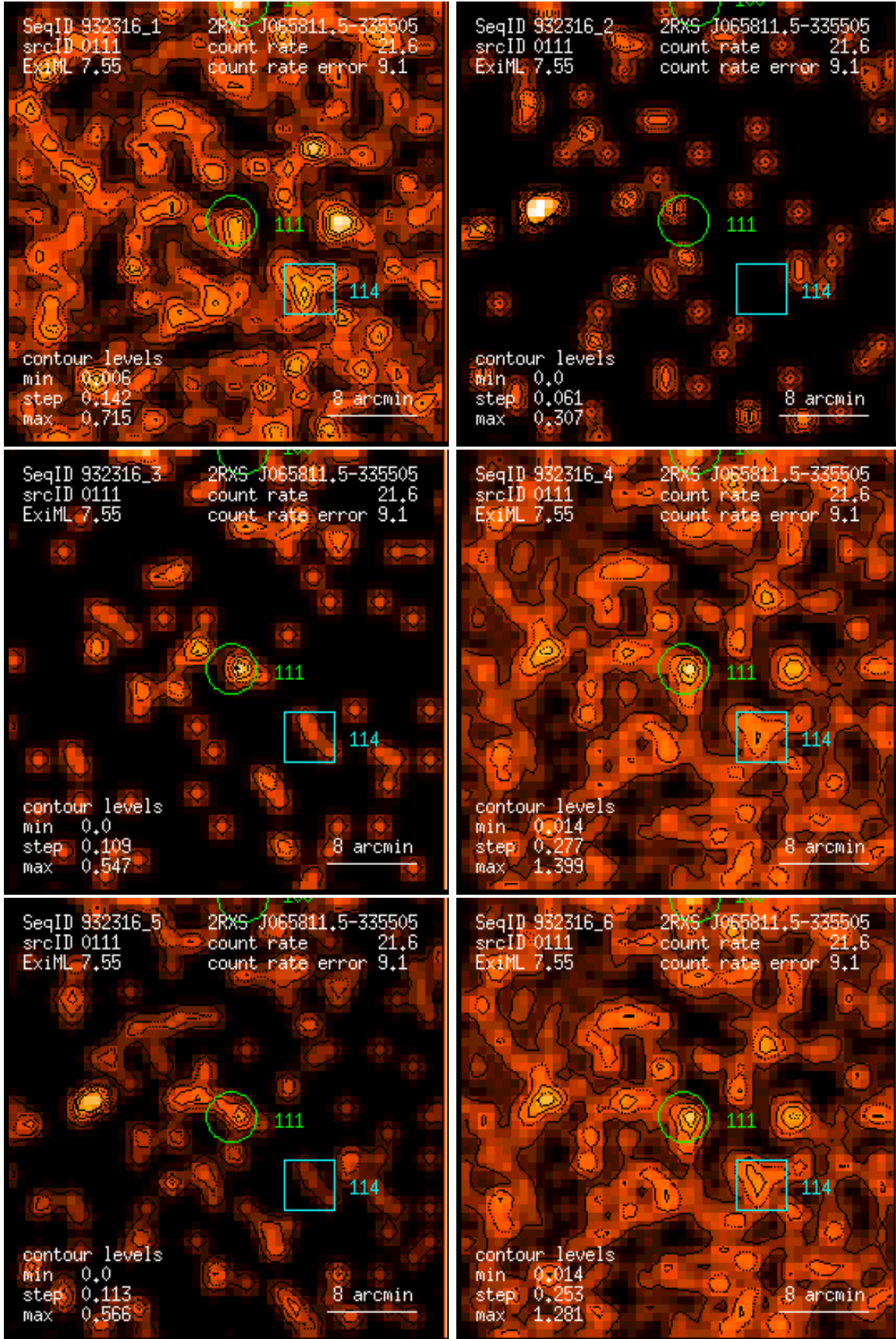
Figure 111: RASS 932316: detection 0111: band rate images, Gaussian filter: (1) PSPC channels 11 – 41, (2) 52 – 90, (3) 91 – 201, (4) 11 – 235, (5) 52 – 201, (6) 11 – 201. Broad band rates in counts/ks. Band rate contour levels in counts/ks/arcmin 2 .
