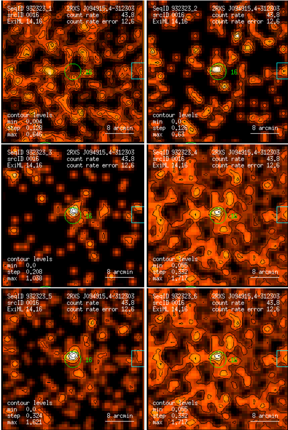
Figure 16: RASS 932323: detection 0016: band rate images, Gaussian filter: (1) PSPC channels 11 – 41, (2) 52 – 90, (3) 91 – 201, (4) 11 – 235, (5) 52 – 201, (6) 11 – 201. Broad band rates in counts/ks. Band rate contour levels in counts/ks/arcmin 2 .
