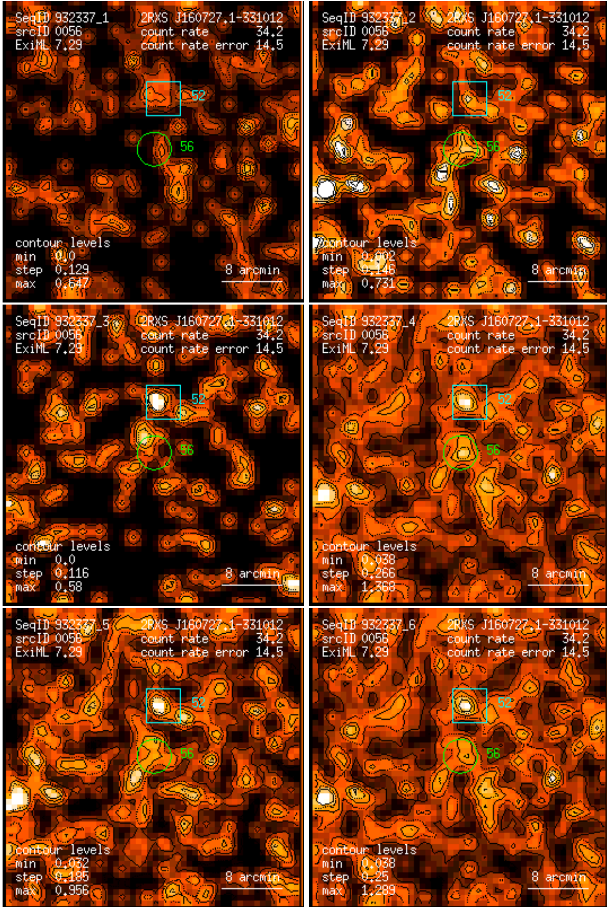
Figure 56: RASS 932337: detection 0056: band rate images, Gaussian filter: (1) PSPC channels 11 – 41, (2) 52 – 90, (3) 91 – 201, (4) 11 – 235, (5) 52 – 201, (6) 11 – 201. Broad band rates in counts/ks. Band rate contour levels in counts/ks/arcmin 2 .
