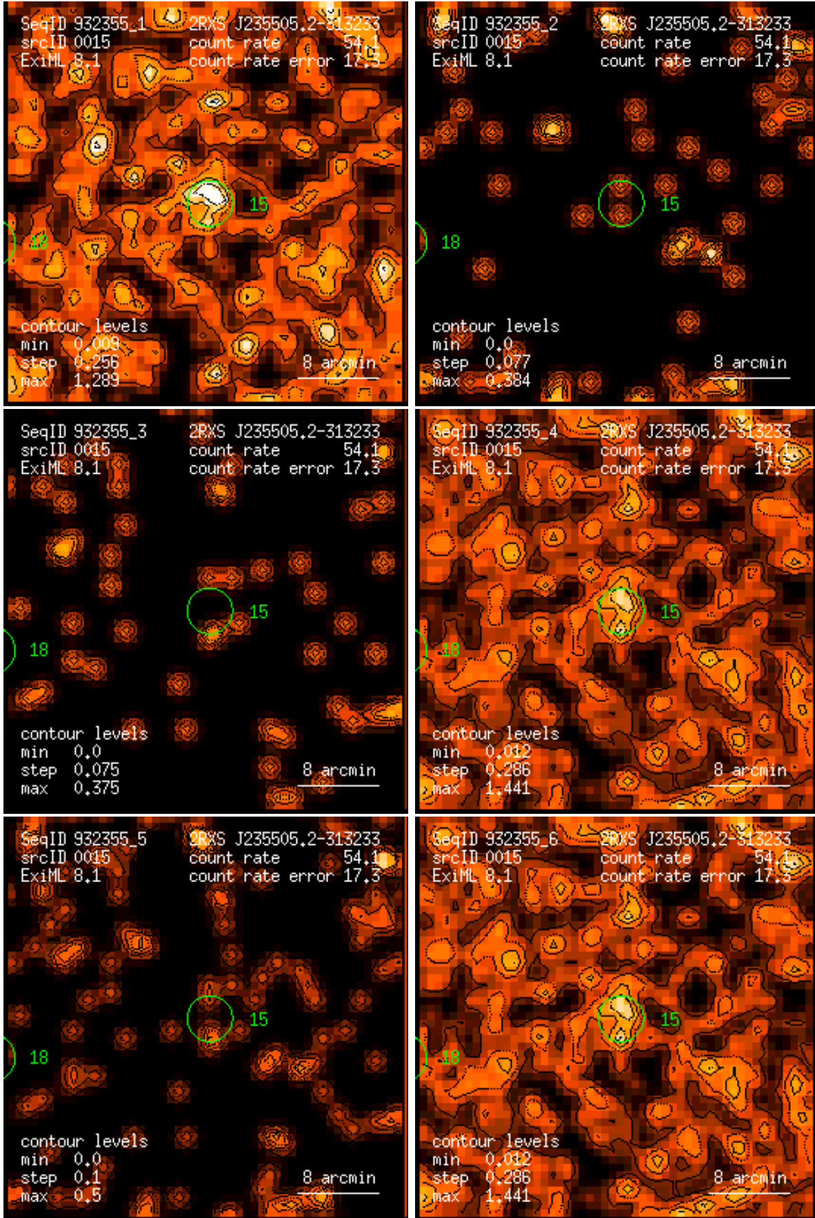
Figure 15: RASS 932355: detection 0015: band rate images, Gaussian filter: (1) PSPC channels 11 – 41, (2) 52 – 90, (3) 91 – 201, (4) 11 – 235, (5) 52 – 201, (6) 11 – 201. Broad band rates in counts/ks. Band rate contour levels in counts/ks/arcmin 2 .
