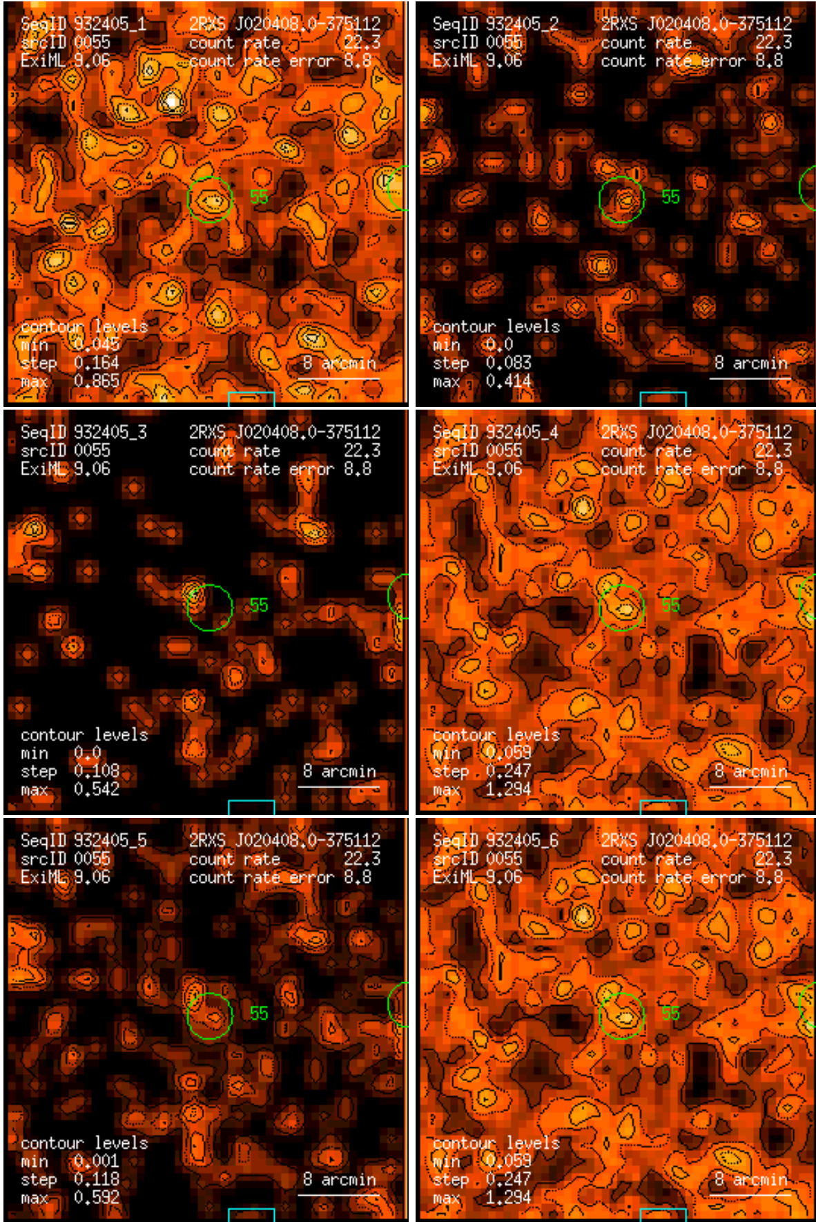
Figure 55: RASS 932405: detection 0055: band rate images, Gaussian filter: (1) PSPC channels 11 – 41, (2) 52 – 90, (3) 91 – 201, (4) 11 – 235, (5) 52 – 201, (6) 11 – 201. Broad band rates in counts/ks. Band rate contour levels in counts/ks/arcmin 2 .
