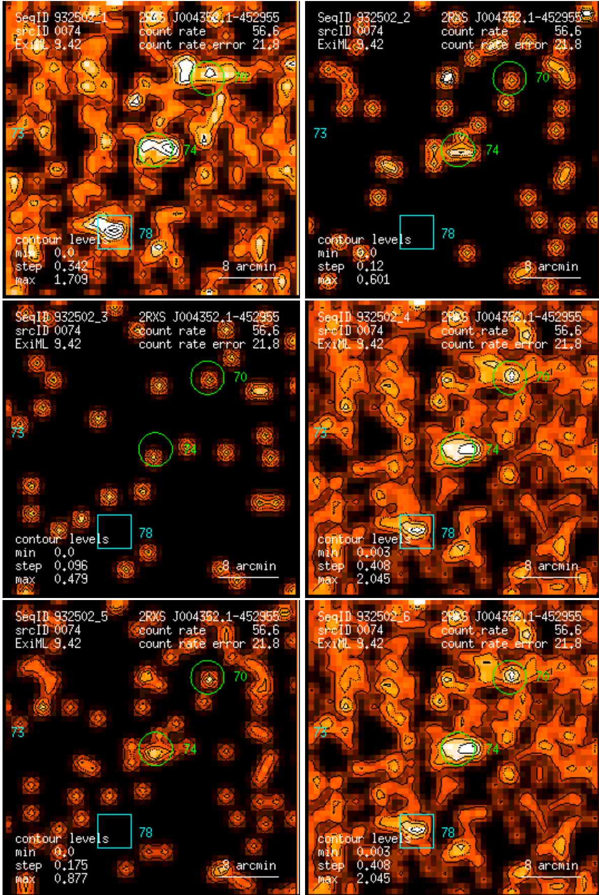
Figure 74: RASS 932502: detection 0074: band rate images, Gaussian filter: (1) PSPC channels 11 – 41, (2) 52 – 90, (3) 91 – 201, (4) 11 – 235, (5) 52 – 201, (6) 11 – 201. Broad band rates in counts/ks. Band rate contour levels in counts/ks/arcmin 2 .
