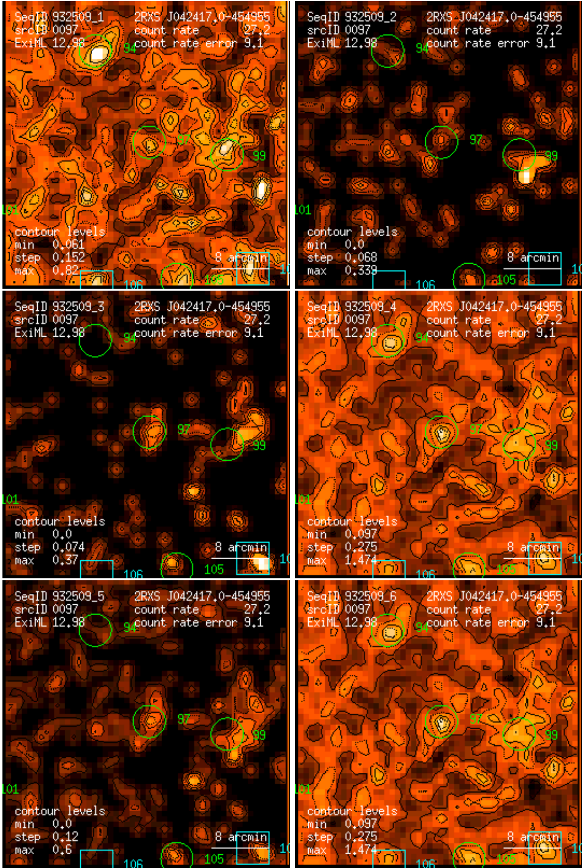
Figure 97: RASS 932509: detection 0097: band rate images, Gaussian filter: (1) PSPC channels 11 – 41, (2) 52 – 90, (3) 91 – 201, (4) 11 – 235, (5) 52 – 201, (6) 11 – 201. Broad band rates in counts/ks. Band rate contour levels in counts/ks/arcmin 2 .
