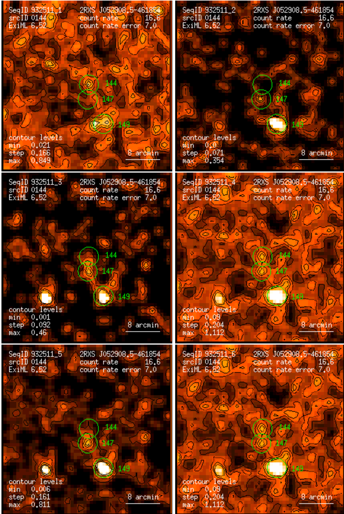
Figure 144: RASS 932511: detection 0144: band rate images, Gaussian filter: (1) PSPC channels 11 – 41, (2) 52 – 90, (3) 91 – 201, (4) 11 – 235, (5) 52 – 201, (6) 11 – 201. Broad band rates in counts/ks. Band rate contour levels in counts/ks/arcmin 2 .
