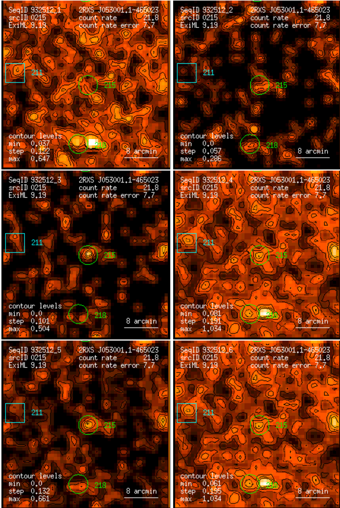
Figure 215: RASS 932512: detection 0215: band rate images, Gaussian filter: (1) PSPC channels 11 – 41, (2) 52 – 90, (3) 91 – 201, (4) 11 – 235, (5) 52 – 201, (6) 11 – 201. Broad band rates in counts/ks. Band rate contour levels in counts/ks/arcmin 2 .
