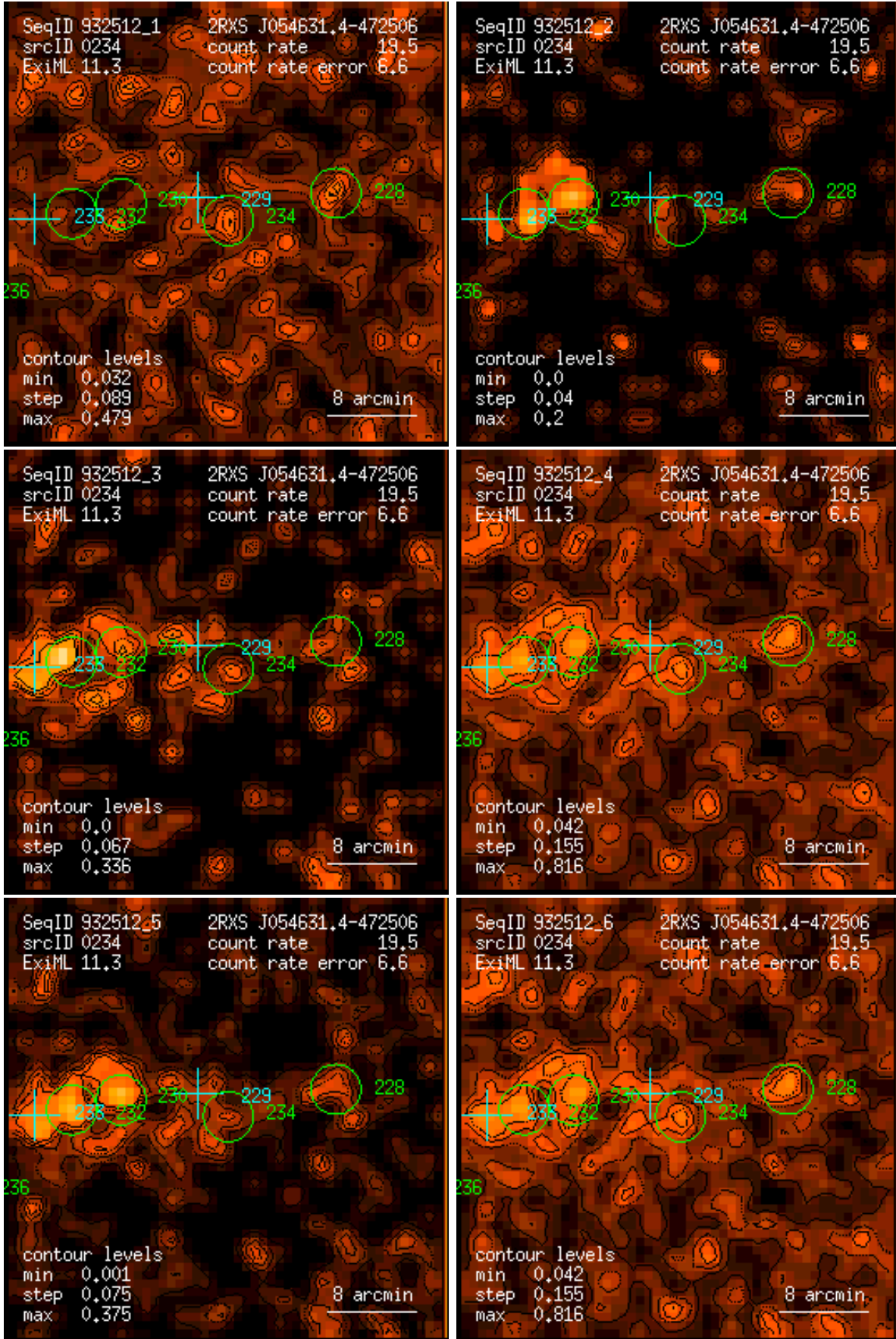
Figure 234: RASS 932512: detection 0234: band rate images, Gaussian filter: (1) PSPC channels 11 – 41, (2) 52 – 90, (3) 91 – 201, (4) 11 – 235, (5) 52 – 201, (6) 11 – 201. Broad band rates in counts/ks. Band rate contour levels in counts/ks/arcmin 2 .
