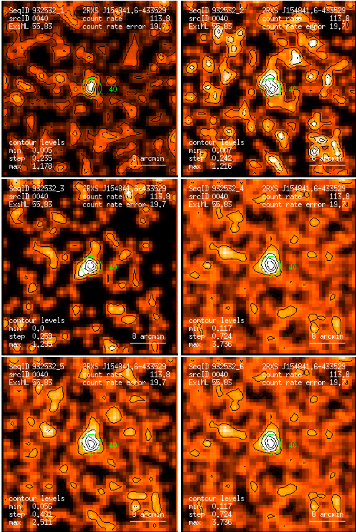
Figure 40: RASS 932532: detection 0040: band rate images, Gaussian filter: (1) PSPC channels 11 – 41, (2) 52 – 90, (3) 91 – 201, (4) 11 – 235, (5) 52 – 201, (6) 11 – 201. Broad band rates in counts/ks. Band rate contour levels in counts/ks/arcmin 2 .
