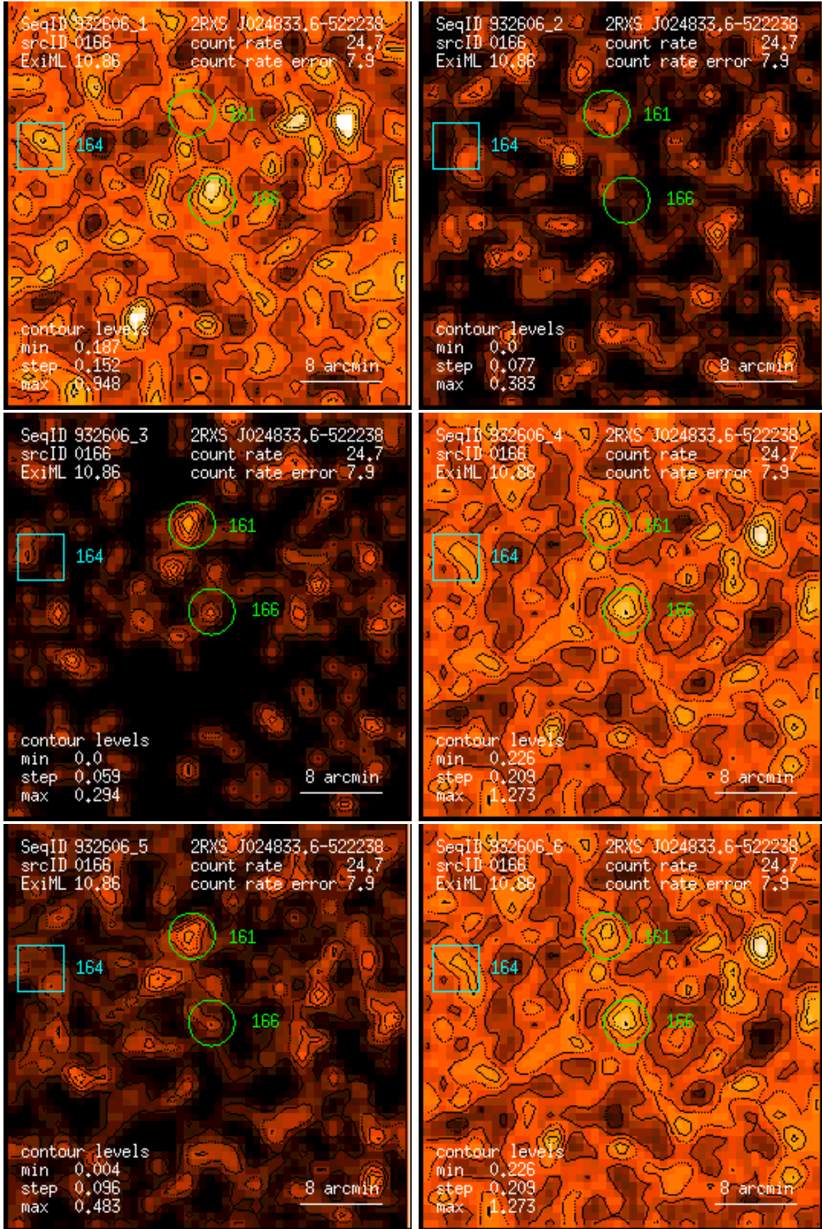
Figure 166: RASS 932606: detection 0166: band rate images, Gaussian filter: (1) PSPC channels 11 – 41, (2) 52 – 90, (3) 91 – 201, (4) 11 – 235, (5) 52 – 201, (6) 11 – 201. Broad band rates in counts/ks. Band rate contour levels in counts/ks/arcmin 2 .
