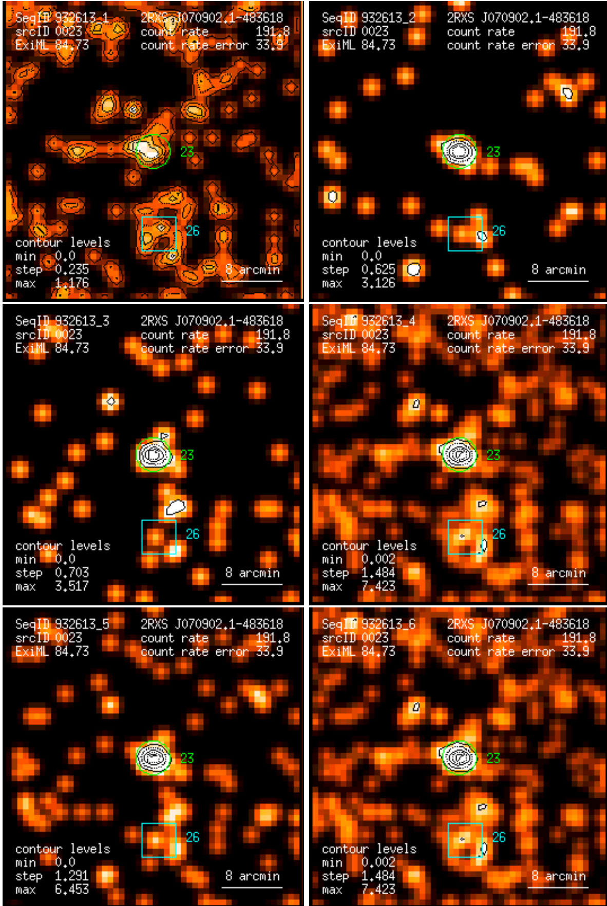
Figure 23: RASS 932613: detection 0023: band rate images, Gaussian filter: (1) PSPC channels 11 – 41, (2) 52 – 90, (3) 91 – 201, (4) 11 – 235, (5) 52 – 201, (6) 11 – 201. Broad band rates in counts/ks. Band rate contour levels in counts/ks/arcmin 2 .
