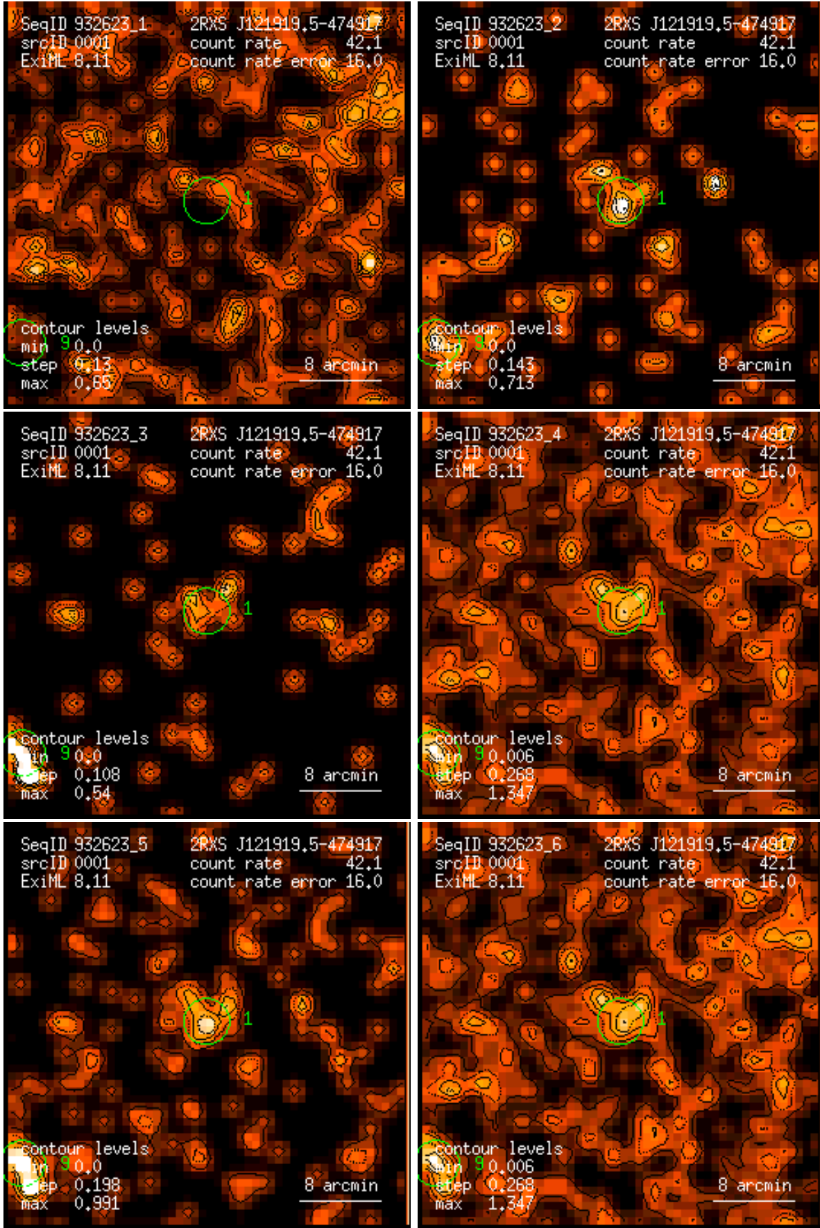
Figure 1: RASS 932623: detection 0001: band rate images, Gaussian filter: (1) PSC channels 11 – 41, (2) 52 – 90, (3) 91 – 201, (4) 11 – 235, (5) 52 – 201, (6) 11 – 201. Broad band rates in counts/ks. Band rate contour levels in counts/ks/arcmin 2 .
