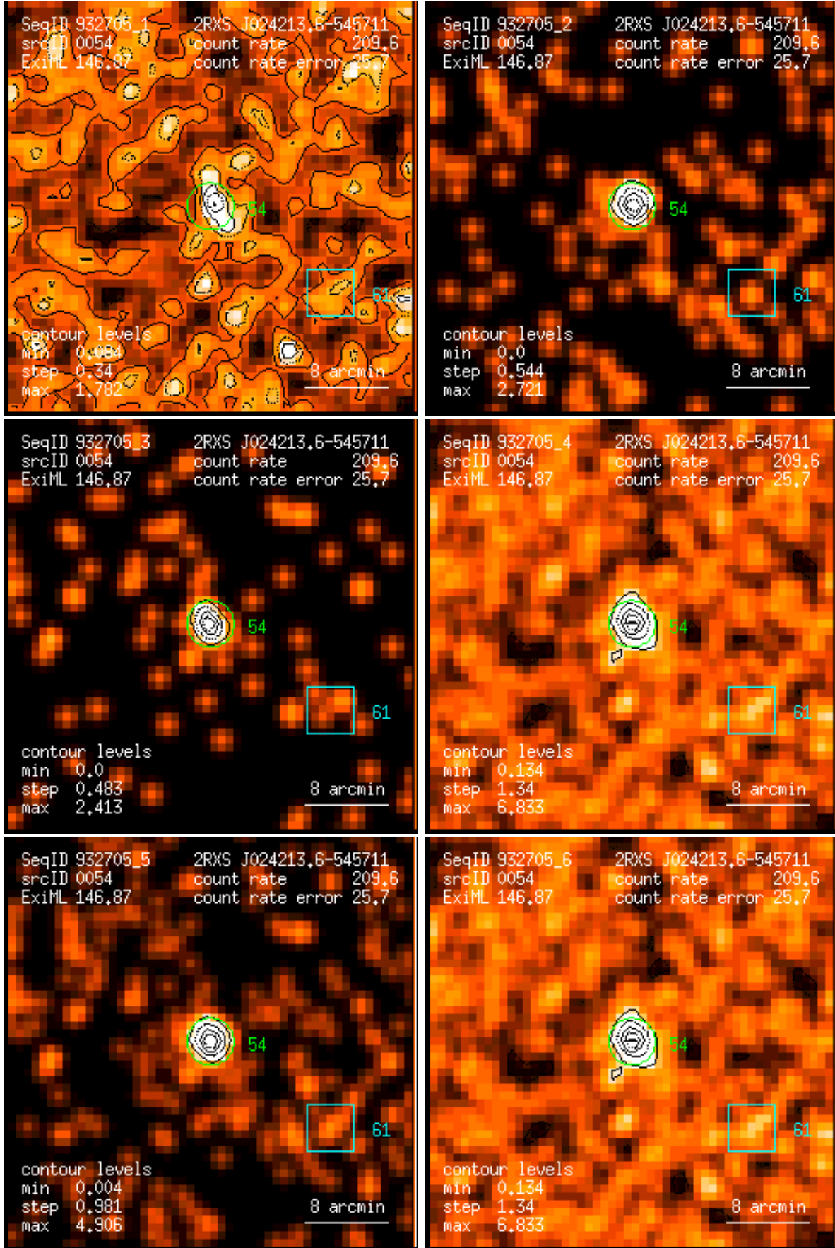
Figure 54: RASS 932705: detection 0054: band rate images, Gaussian filter: (1) PSPC channels 11 – 41, (2) 52 – 90, (3) 91 – 201, (4) 11 – 235, (5) 52 – 201, (6) 11 – 201. Broad band rates in counts/ks. Band rate contour levels in counts/ks/arcmin 2 .
