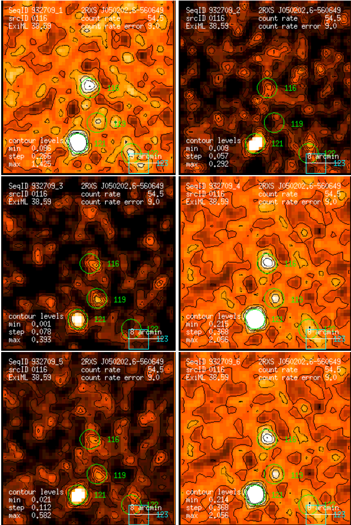
Figure 116: RASS 932709: detection 0116: band rate images, Gaussian filter: (1) PSPC channels 11 – 41, (2) 52 – 90, (3) 91 – 201, (4) 11 – 235, (5) 52 – 201, (6) 11 – 201. Broad band rates in counts/ks. Band rate contour levels in counts/ks/arcmin 2 .
