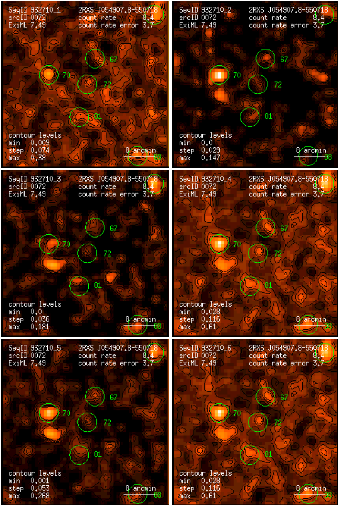
Figure 72: RASS 932710: detection 0072: band rate images, Gaussian filter: (1) PSPC channels 11 – 41, (2) 52 – 90, (3) 91 – 201, (4) 11 – 235, (5) 52 – 201, (6) 11 – 201. Broad band rates in counts/ks. Band rate contour levels in counts/ks/arcmin 2 .
