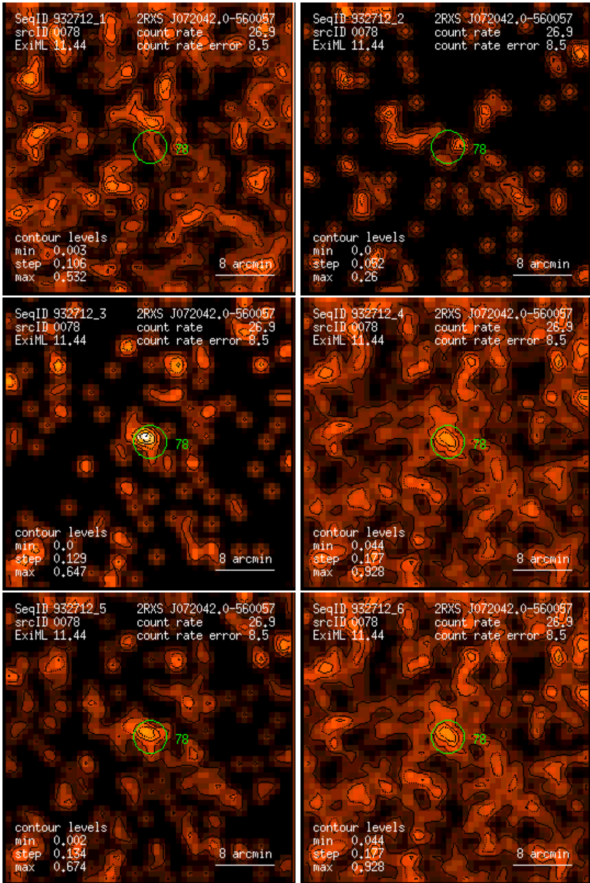
Figure 78: RASS 932712: detection 0078: band rate images, Gaussian filter: (1) PSPC channels 11 – 41, (2) 52 – 90, (3) 91 – 201, (4) 11 – 235, (5) 52 – 201, (6) 11 – 201. Broad band rates in counts/ks. Band rate contour levels in counts/ks/arcmin 2 .
