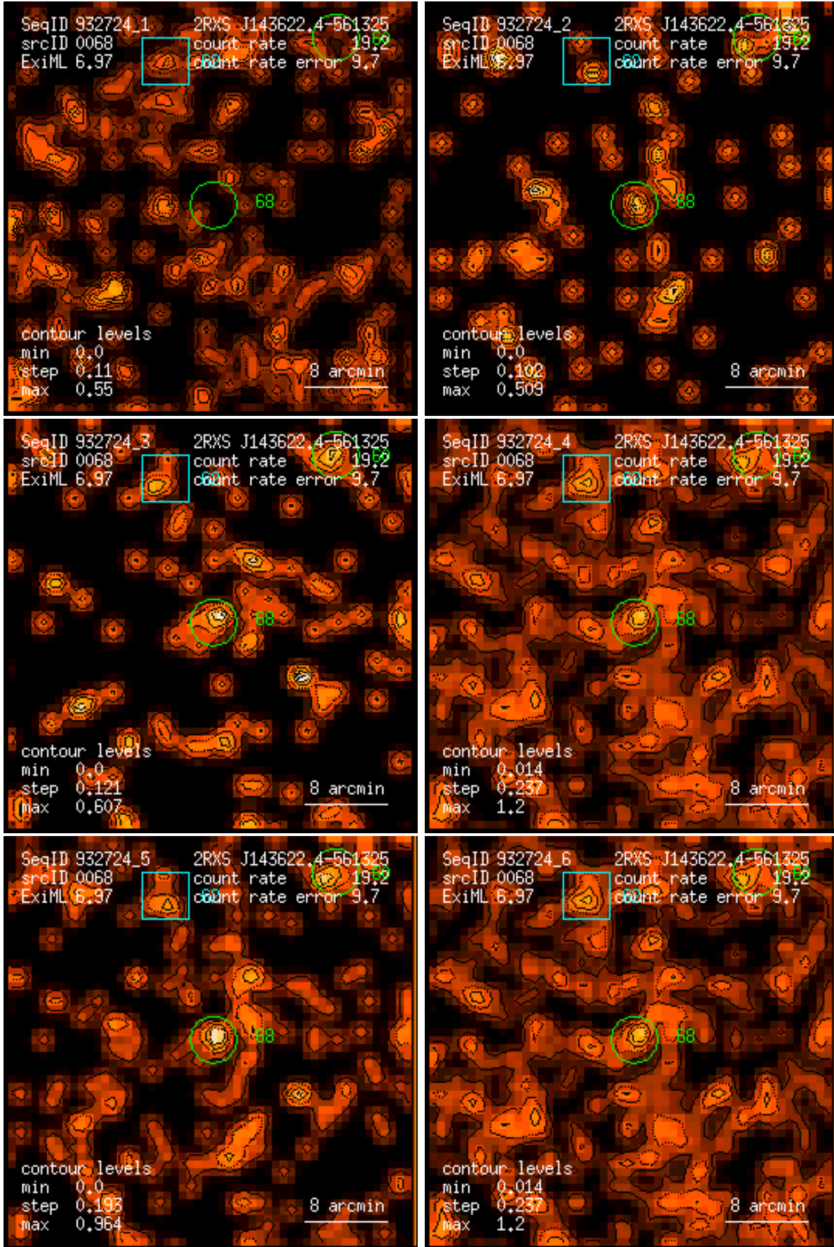
Figure 68: RASS 932724: detection 0068: band rate images, Gaussian filter: (1) PSPC channels 11 – 41, (2) 52 – 90, (3) 91 – 201, (4) 11 – 235, (5) 52 – 201, (6) 11 – 201. Broad band rates in counts/ks. Band rate contour levels in counts/ks/arcmin 2 .
