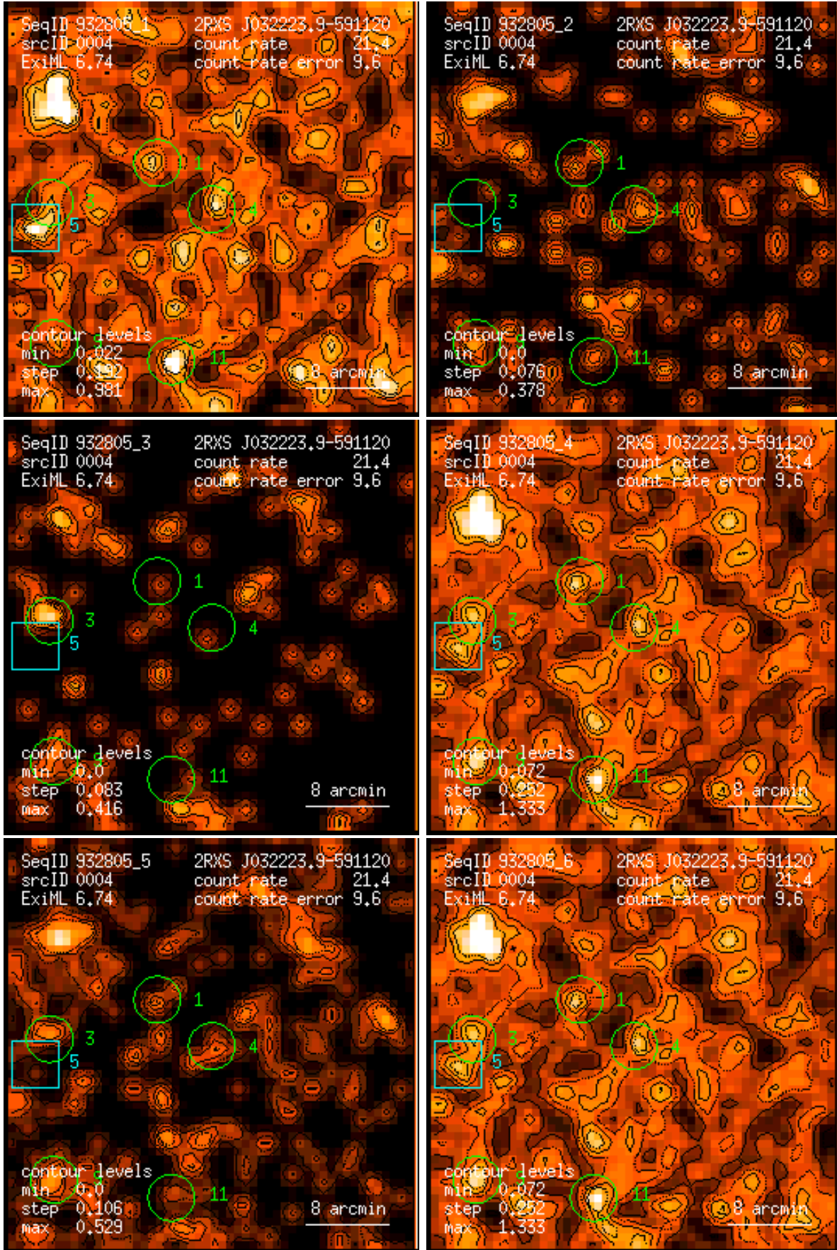
Figure 4: RASS 932805: detection 0004: band rate images, Gaussian filter: (1) PSPC channels 11 – 41, (2) 52 – 90, (3) 91 – 201, (4) 11 – 235, (5) 52 – 201, (6) 11 – 201. Broad band rates in counts/ks. Band rate contour levels in counts/ks/arcmin 2 .
