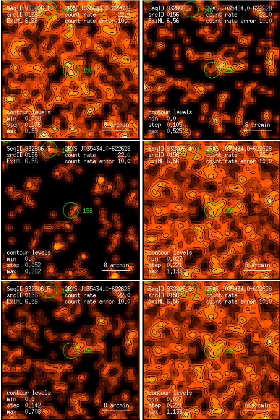
Figure 156: RASS 932806: detection 0156: band rate images, Gaussian filter: (1) PSPC channels 11 – 41, (2) 52 – 90, (3) 91 – 201, (4) 11 – 235, (5) 52 – 201, (6) 11 – 201. Broad band rates in counts/ks. Band rate contour levels in counts/ks/arcmin 2 .
