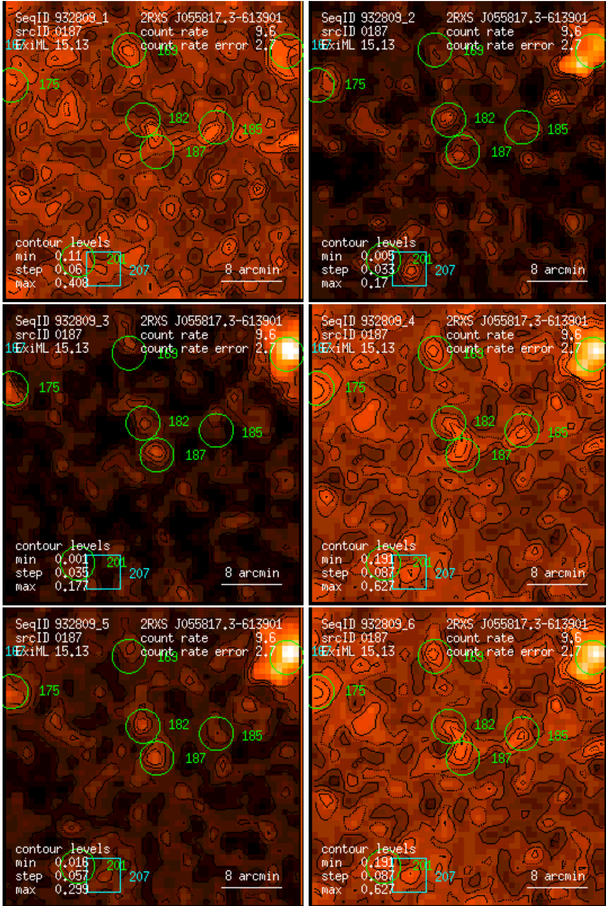
Figure 187: RASS 932809: detection 0187: band rate images, Gaussian filter: (1) PSPC channels 11 – 41, (2) 52 – 90, (3) 91 – 201, (4) 11 – 235, (5) 52 – 201, (6) 11 – 201. Broad band rates in counts/ks. Band rate contour levels in counts/ks/arcmin 2 .
