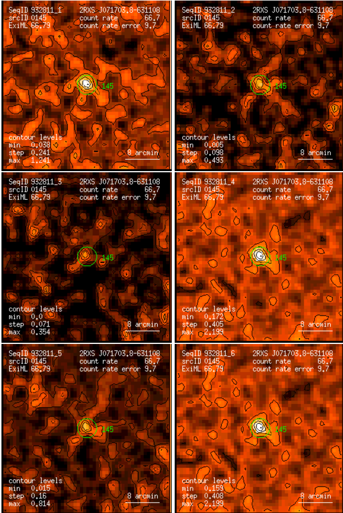
Figure 145: RASS 932811: detection 0145: band rate images, Gaussian filter: (1) PSPC channels 11 – 41, (2) 52 – 90, (3) 91 – 201, (4) 11 – 235, (5) 52 – 201, (6) 11 – 201. Broad band rates in counts/ks. Band rate contour levels in counts/ks/arcmin 2 .
