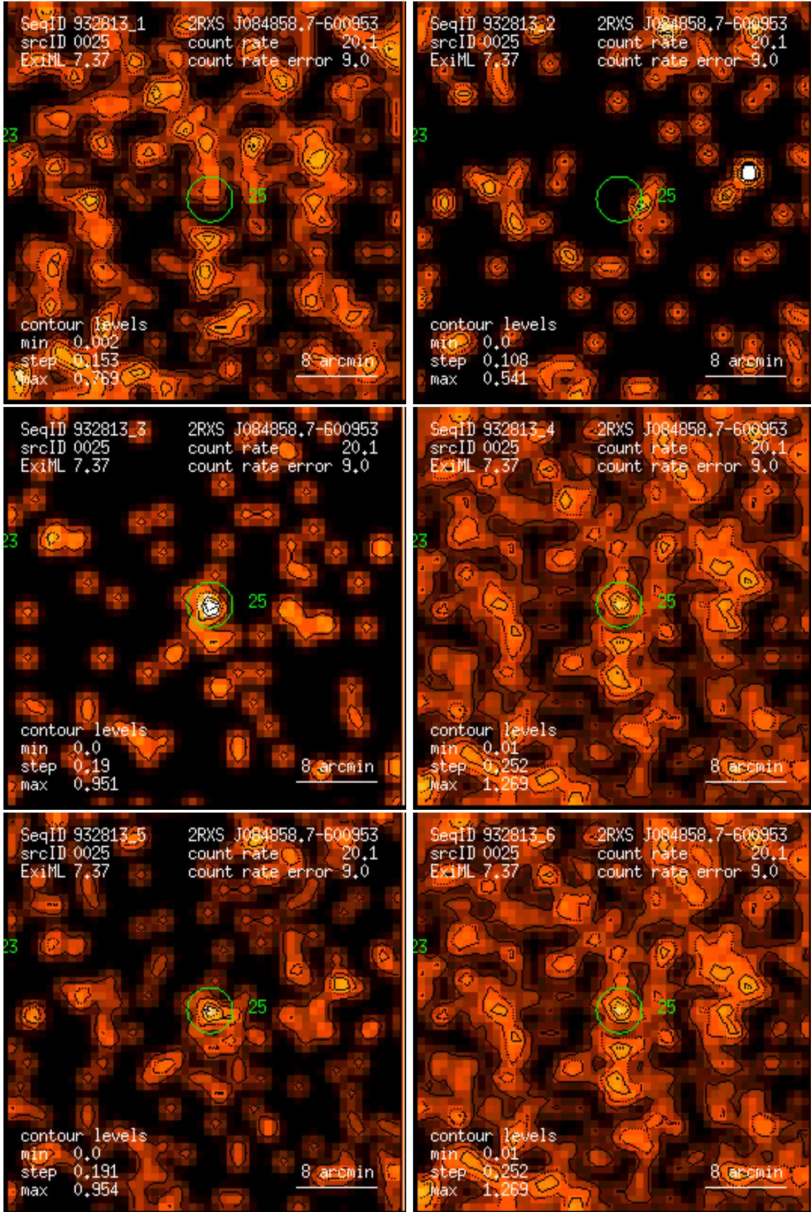
Figure 25: RASS 932813: detection 0025: band rate images, Gaussian filter: (1) PSPC channels 11 – 41, (2) 52 – 90, (3) 91 – 201, (4) 11 – 235, (5) 52 – 201, (6) 11 – 201. Broad band rates in counts/ks. Band rate contour levels in counts/ks/arcmin 2 .
