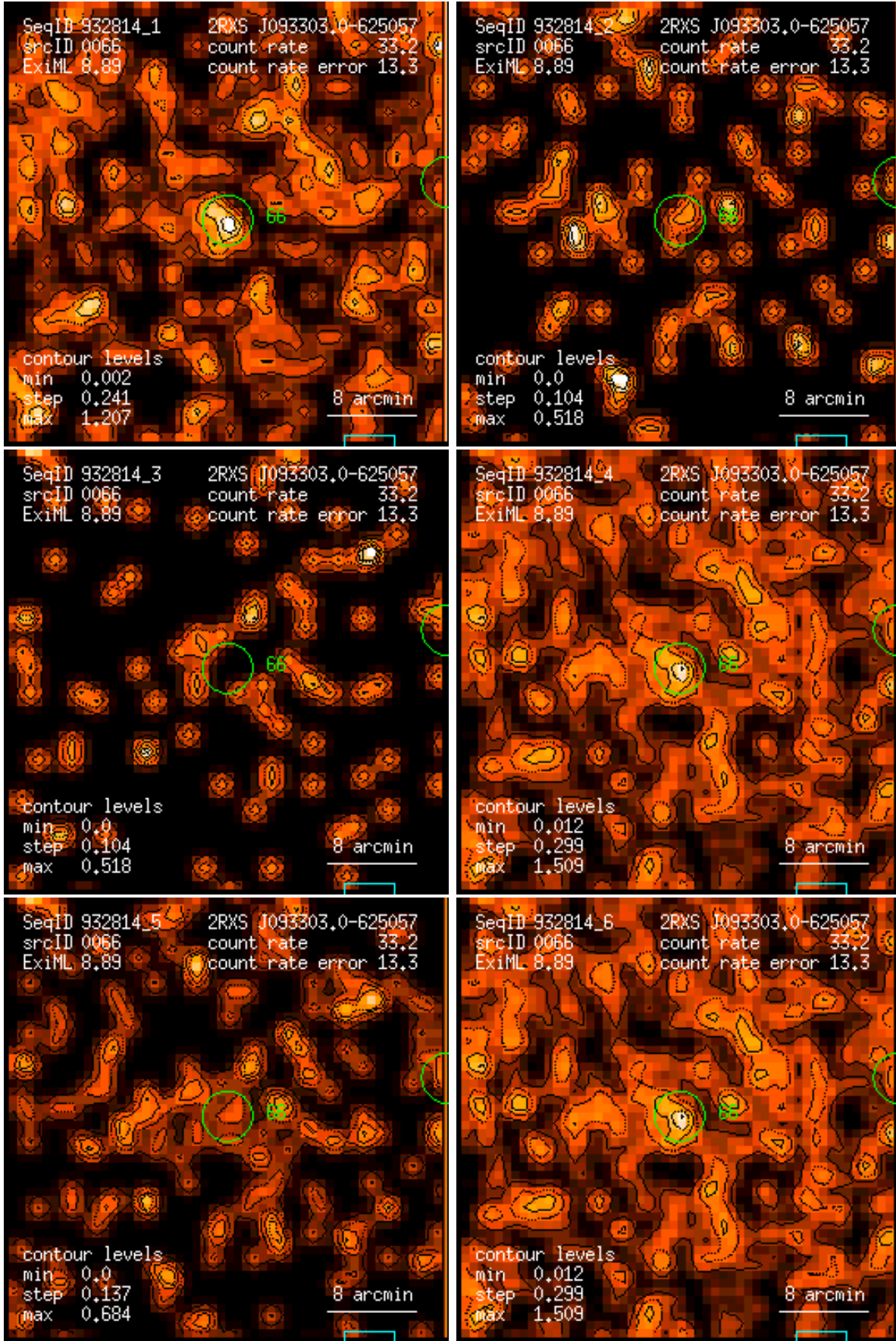
Figure 66: RASS 932814: detection 0066: band rate images, Gaussian filter: (1) PSPC channels 11 – 41, (2) 52 – 90, (3) 91 – 201, (4) 11 – 235, (5) 52 – 201, (6) 11 – 201. Broad band rates in counts/ks. Band rate contour levels in counts/ks/arcmin 2 .
