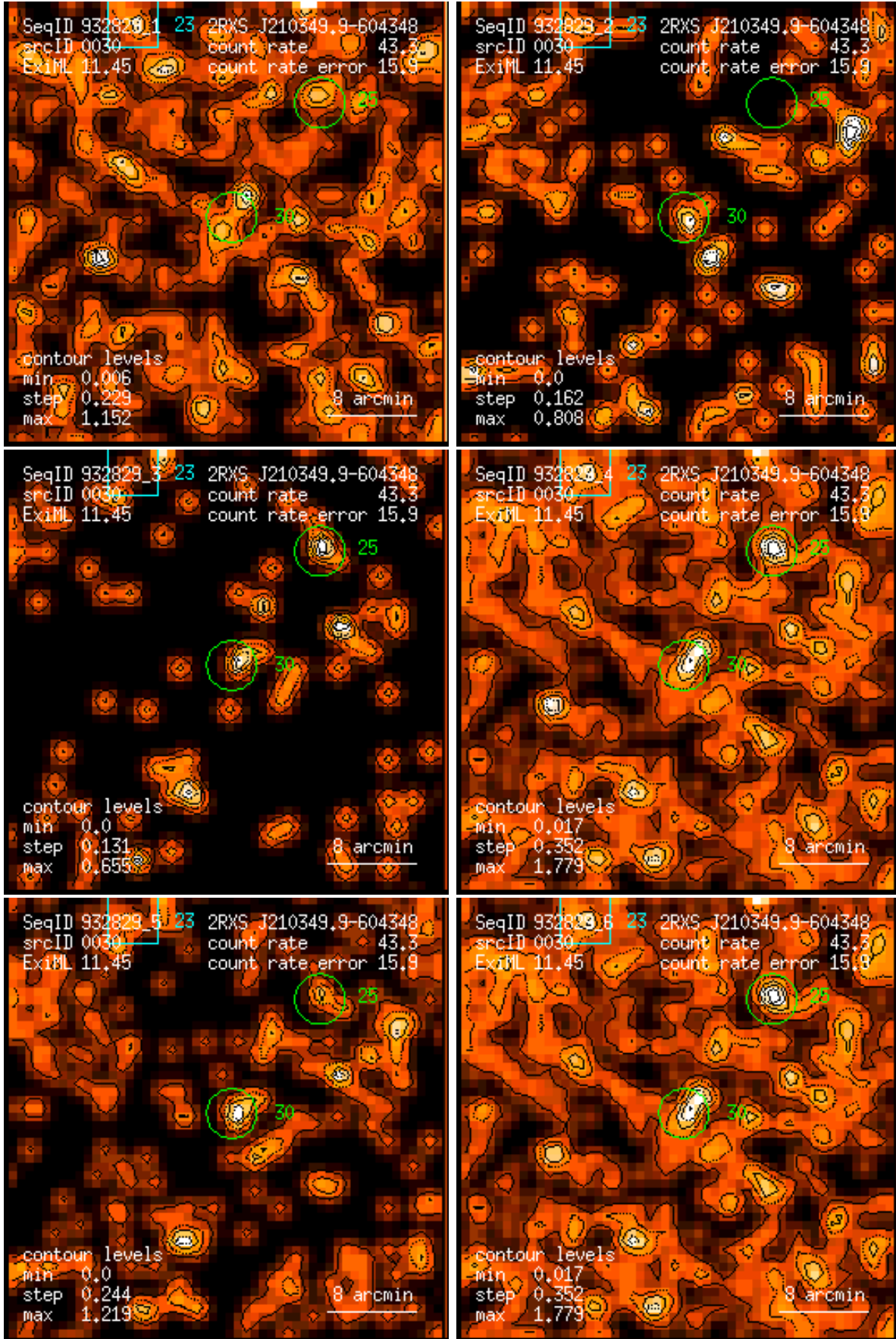
Figure 30: RASS 932829: detection 0030: band rate images, Gaussian filter: (1) PSPC channels 11 – 41, (2) 52 – 90, (3) 91 – 201, (4) 11 – 235, (5) 52 – 201, (6) 11 – 201. Broad band rates in counts/ks. Band rate contour levels in counts/ks/arcmin 2 .
